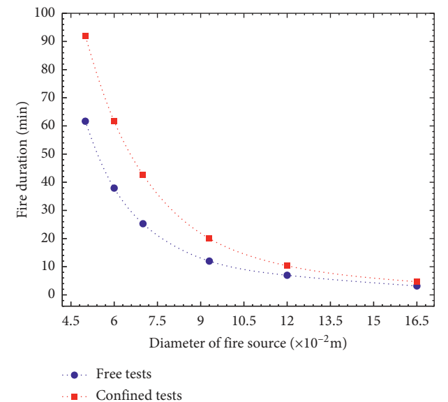
FIGURE 13: Variation of the duration of fire in opened and confined surroundings.
