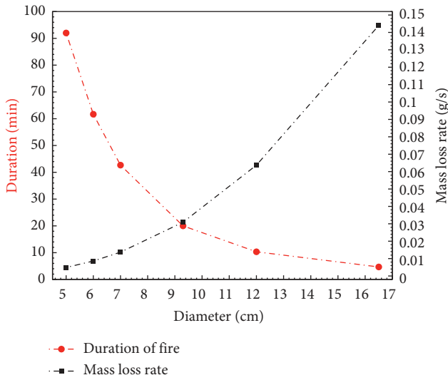
FIGURE 10: Variation of the fire duration and mass loss rate of fuel according to the source: case of confined tests.
