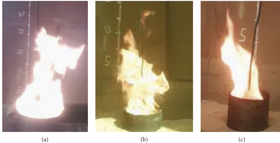
FIGURE 3: Images of flame during free fires: (a) source 1, (b) source 3, and (c) source 5.
