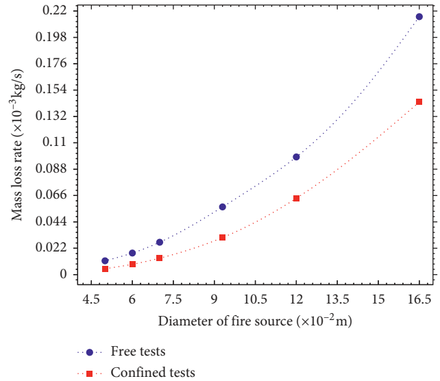
FIGURE 12: Variation of the mass loss rate of fuel in opened and confined surroundings.
