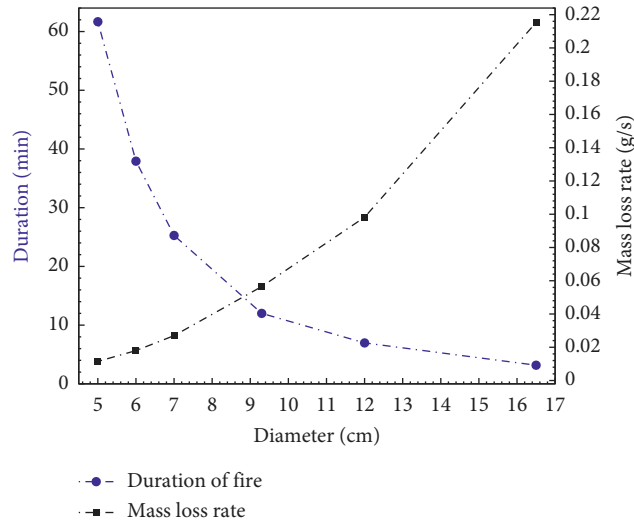
FIGURE 6: Variation of the fire duration and the fuel mass loss rate according to the fire source: case of fire in free atmosphere.
