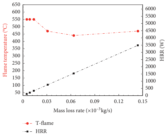
FIGURE 11: Variation of the flame temperature and heat release rate according to the mass loss rate: case of confined tests.
