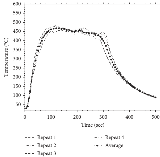
FIGURE 8: Evolution of temperature in the persistent zone of the flame during the four repeated tests: case of source 1.
