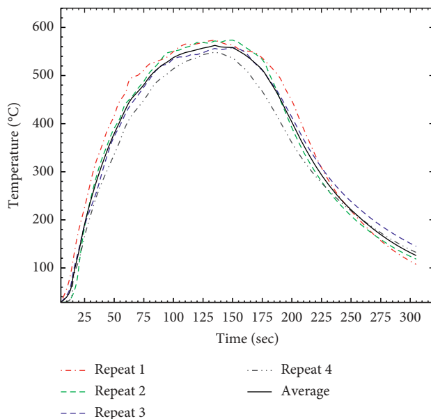
FIGURE 4: Flame temperature versus time: case study of free fire with fire source 1.
