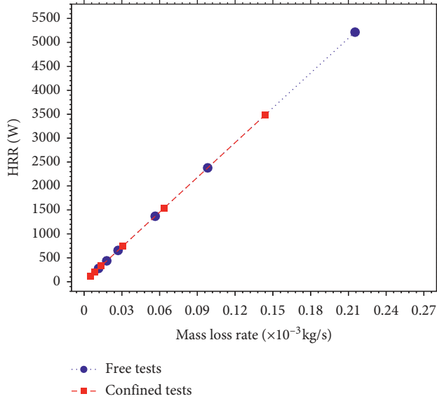
FIGURE 14: Variation of the heat release rate in open and confined surroundings.
