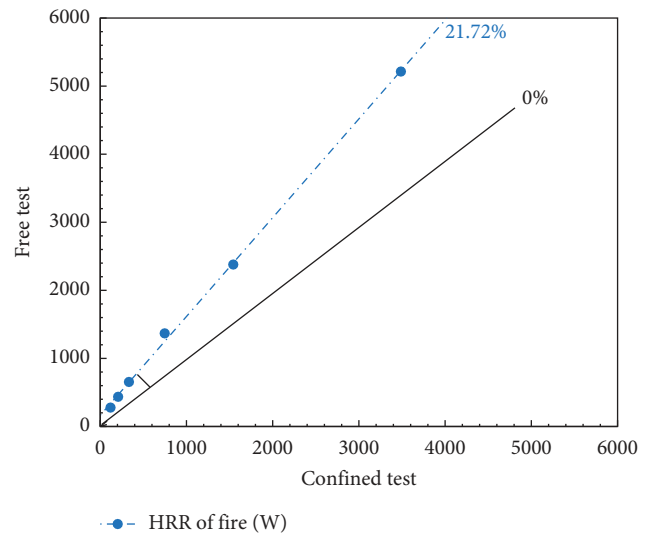
FIGURE 17: Angle of the shift of the effect of confining on the heat release rate of the fire source.
