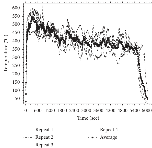
FIGURE 9: Evolution of temperature in the persistent zone of the flame during the four repeated tests: case of source 6.
