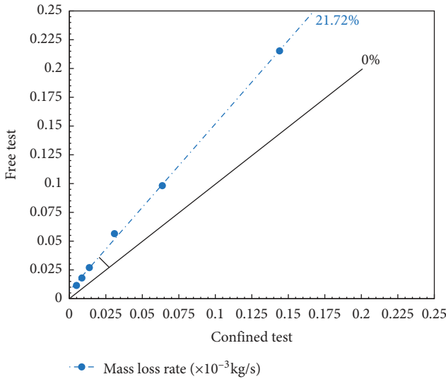
FIGURE 15: Angle of the shift of the effect of confining on the mass loss rate of fuel.
