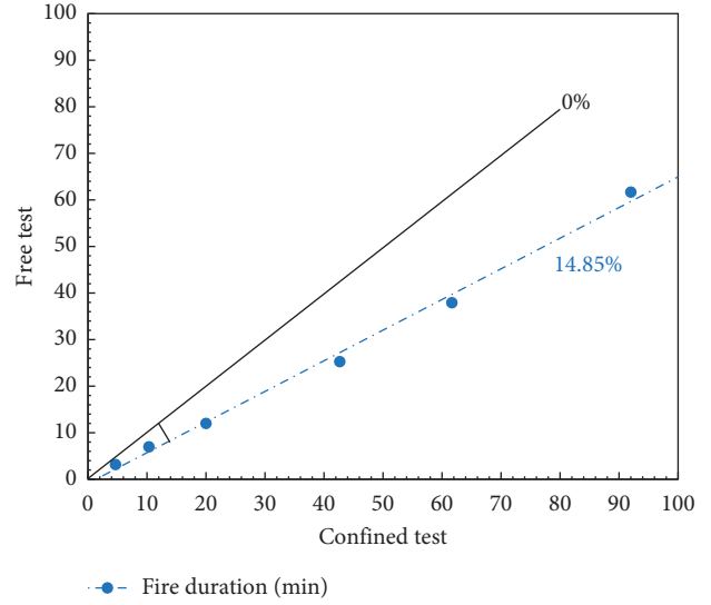
FIGURE 16: Angle of the shift of the effect of confining on the duration of fire.
