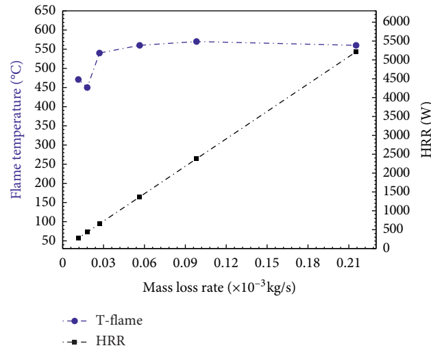
FIGURE 7: Variation of the flame temperature and the heat release rate according to the fire source: case of fire in free atmosphere.
