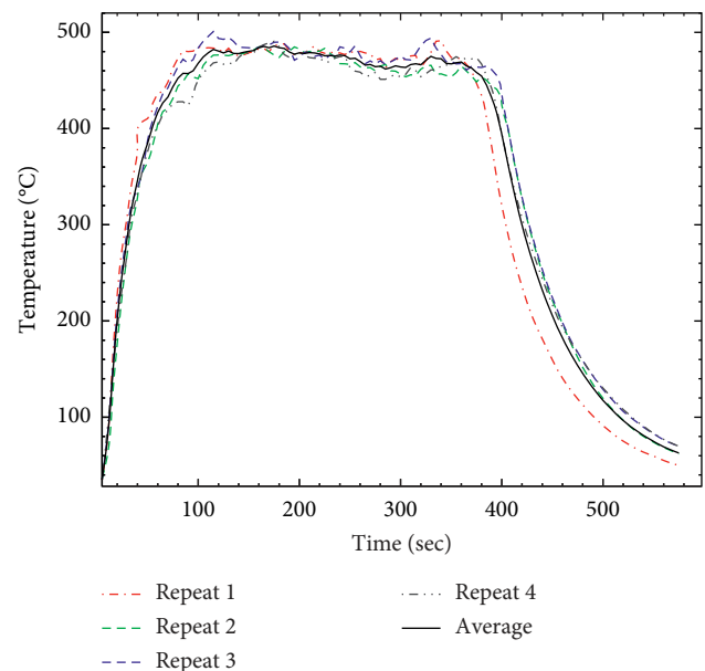
FIGURE 5: Flame temperature versus time: case study of free fire with fire source 6.
