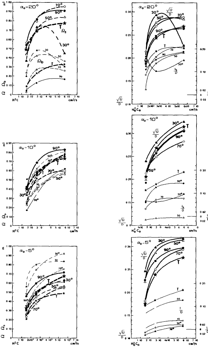
Fig 8 - Curves of the parameter defining the efficiency of groyne in function of the transmitted wave power
