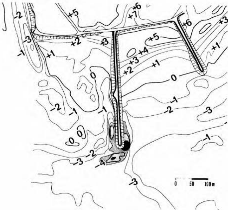
Fig. 17 - Plan of the groynes in Cova do Vapor (September 1969)
