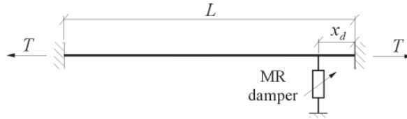
Fig. 1. Cable with an attached MR damper
