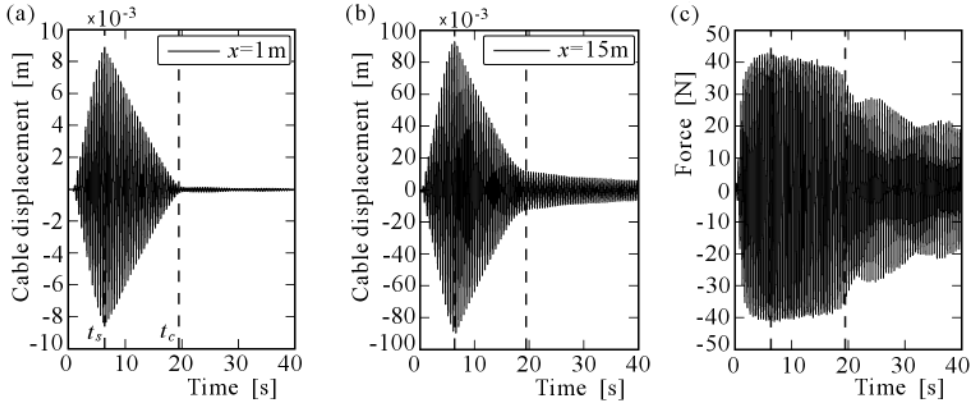
Fig. 10. Free vibration of the cable with the MR damper for I = 0.5\text{ A} : (a) cable displacement at the damper location, (b) cable displacement at the mid-point, (c) force along the damper axis
