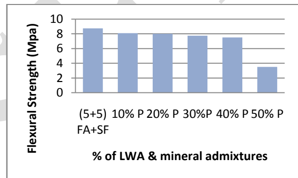
Fig.11 Flexural strength
