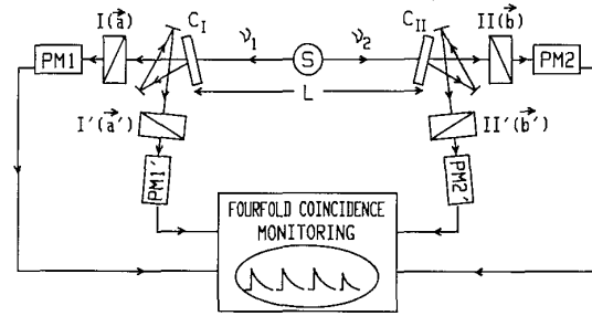
FIG. 2. Timing experiment with optical switches. Each switching device ( C_1, C_2 ) is followed by two polarizers in two different orientations. Each combination is equivalent to a polarizer switched fast between two orientations.
