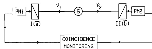
FIG. 1. Optical version of the Einstein-Podolsky-Rosen-Bohm Gedankenexperiment . The pair of photons \nu_1 and \nu_2 is analyzed by linear polarizers I and II (in orientations \vec{a} and \vec{b} ) and photomultipliers. The coincidence rate is monitored.
