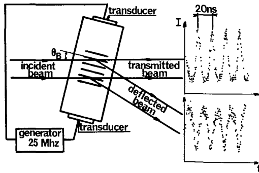
FIG. 3. Optical switch. The incident light is switched at a frequency around 50 MHz by diffraction at the Bragg angle on an ultrasonic standing wave. The intensities of the transmitted and deflected beams as a function of time have been measured with the actual source. The fraction of light directed towards other diffraction orders is negligible.
