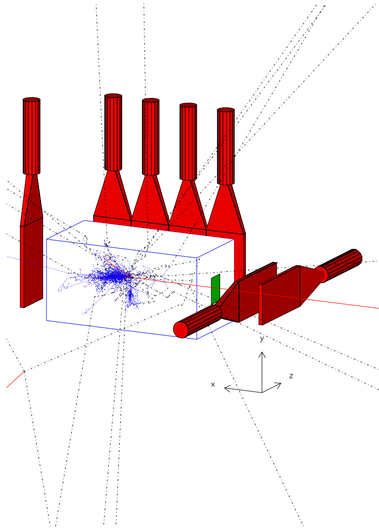
Figure 2: A simulation of a secondary particle cascade produced by 4 GeV/c incoming proton in the 40cm×40cm×80cm iron block with the arrangement of the scintillator detectors.
