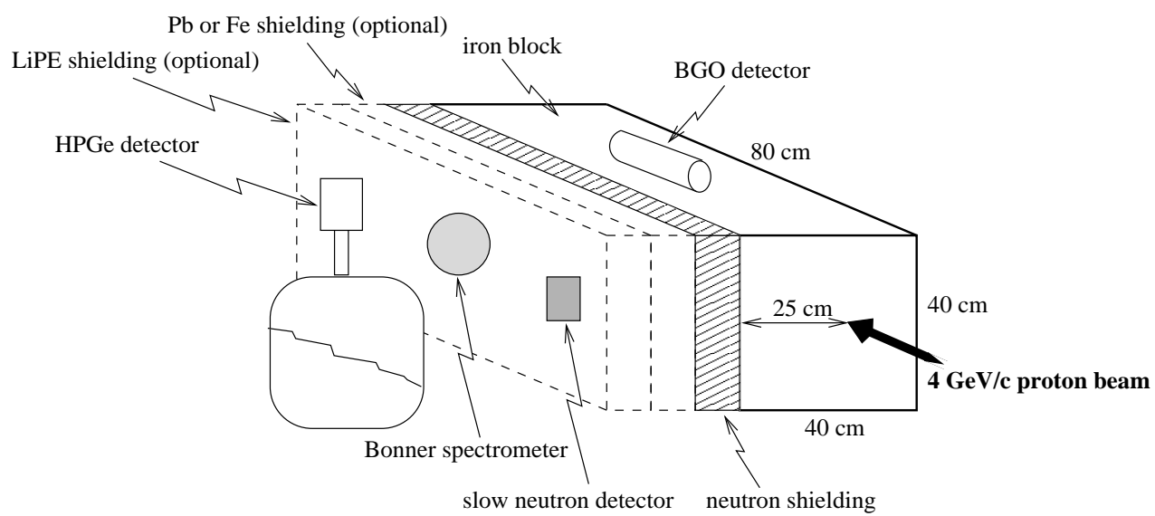
Figure 1: Experimental set-up.
