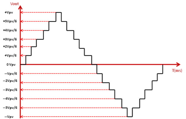
Fig. 4. Modelled 13-level inverter output voltage waveform
