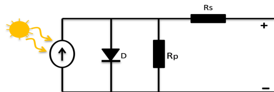
Figure 1. Equivalent Circuit of a PV cell.
