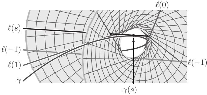
Fig. 3. \ell(s) meets the hyperboloid in two real points.
