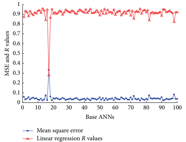
FIGURE 16: MSE and R values of the 100 base ANNs for experiment 1.
