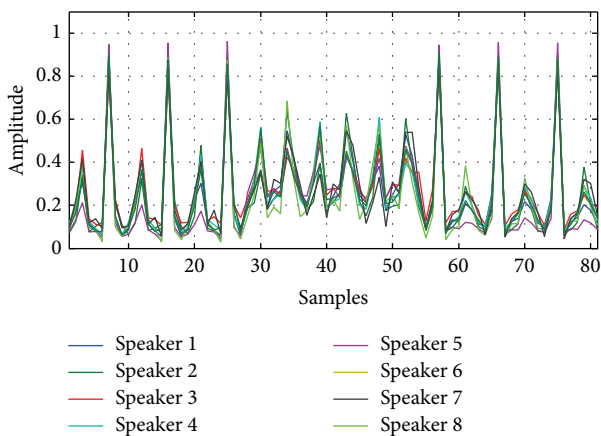
FIGURE 19: Time domain plot of the MFDWC HOG features for the utterance “Hello Hello Hello ...” of the first 8 Speakers.
