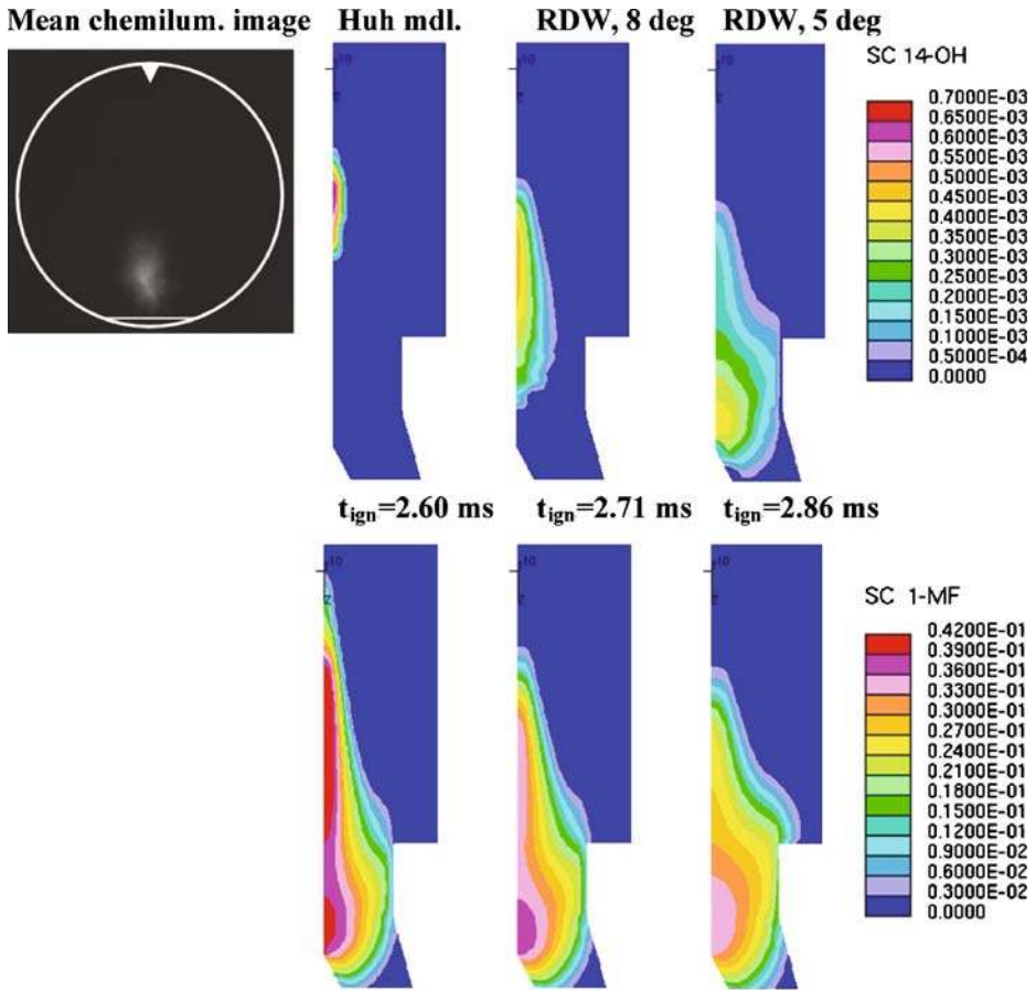
Fig. 20 Ignition location comparison: mean \text{OH}^* chemiluminescence signal averaged from 48 individual realisations 2.5 ms after start of injection ( upper left ); the white circle symbolises the cell window, the straight line at the bottom the location of the wall and the triangle the injector. Simulated OH mass fraction ( upper row ) and mixture fraction ( lower row ) iso-contours at the time of ignition for the Huh model [51], the Reitz–Diwakar Model [52] with 8° and 5° cone angle (from left to right ). The Liu et al. mechanism [59] has been used at the nominal air temperature of 776 K
