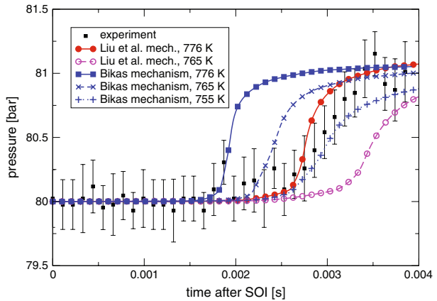
Fig. 14 Pressure variation with time for various initial air temperatures and two chemical mechanisms [58, 59]. The Huh atomisation model [51] has been used
