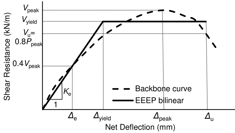
Fig. 11. EEEP Model [19]
