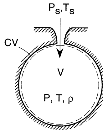
(b) Charge
