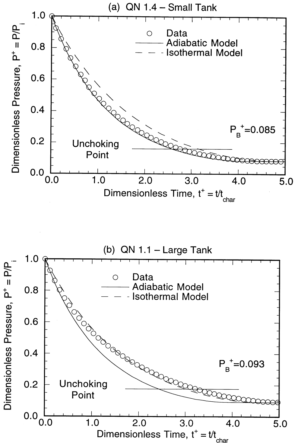
Fig. 4. Example single experiment data for the discharge experiment: (a) nozzle QN1.4—small tank, (b) nozzle QN1.1—large tank; uncertainty in P^+ = \pm 0.0075 and in t^+ = \pm 0.15 to 95% confidence.
