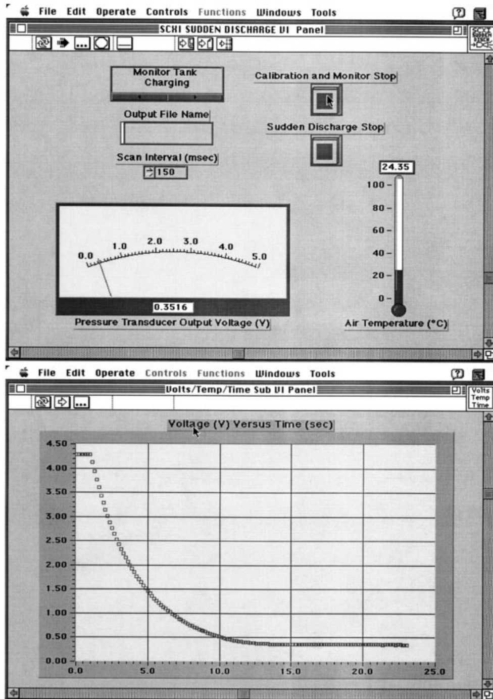
Fig. 3. Reproduction of the LabVIEW front panel for the discharge experiment.
