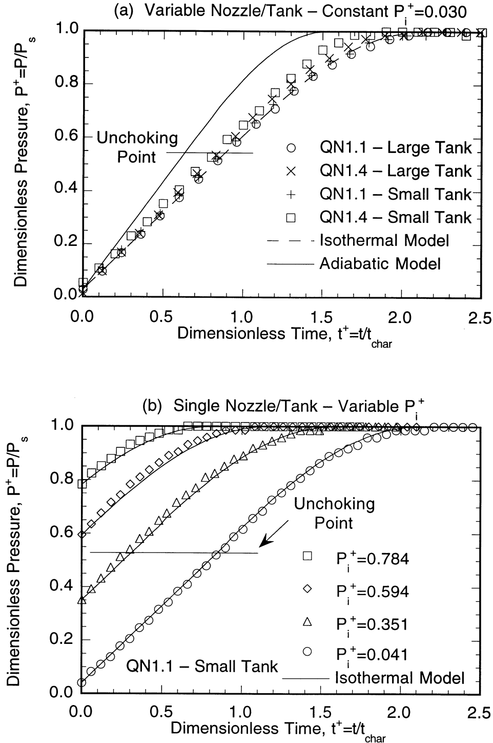
Fig. 7. Example composite data for the filling experiment: (a) variable nozzle/tank combinations and constant P_i^+ , (b) variable P_i^+ and constant nozzle/tank combination; uncertainties same as in Fig. 6.
