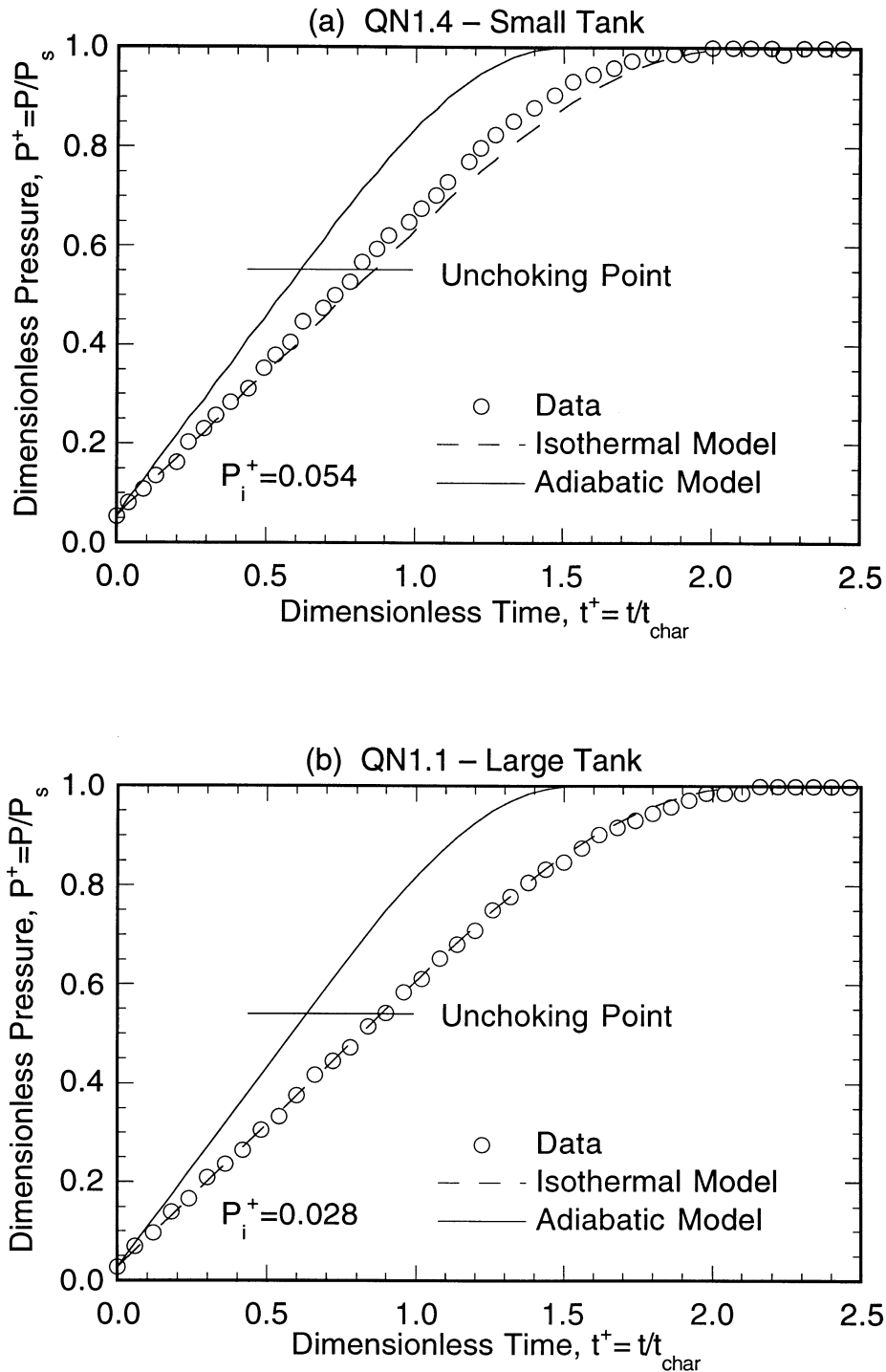
Fig. 6. Example single experiment data for the filling experiment: (a) nozzle QN1.4—small tank, (b) nozzle QN1.1—large tank; uncertainty in P^+ = \pm 0.015 and in t^+ = \pm 0.08 to 95% confidence.
