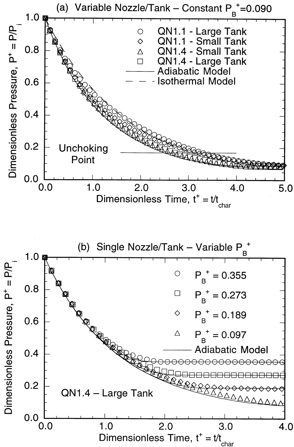
Fig. 5. Example composite data for the discharge experiment: (a) variable nozzle-tank combinations and constant P_B^+ , (b) variable P_B^+ and constant nozzle-tank combination; uncertainties same as in Fig. 4.
