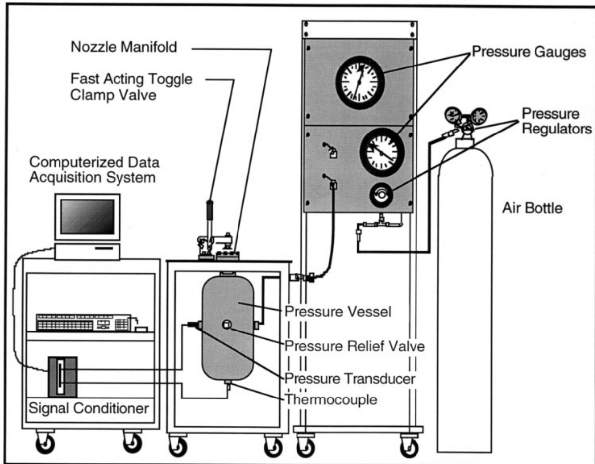
Fig. 2. Schematic diagram of the vessel discharge experimental apparatus.
