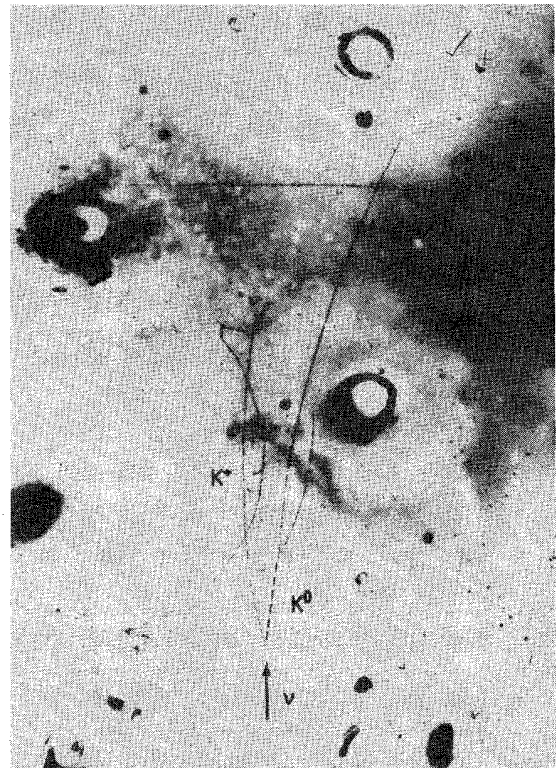
FIG. 7. A "muonless" event in Gargamelle. All tracks stop or interact in the chamber. None could be a muon. The neutrino produces one K^+ and one K^0 meson. The K^+ meson interacts in the liquid and then decays. The invisible K^0 meson decays to two pions.
