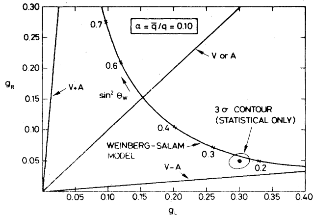
FIG. 10. Strengths of the left- and right-handed neutral currents. If the NC were purely left handed, as is the case for the CC, the experimental point would be expected to fall on the V-A line. The experiment shows a right-handed component, which is just that expected in the electroweak theory (Weinberg-Salam model) (Holder et al. , 1977c).
