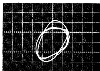
1 CM = 0.5 MILS (B) UNSTABLE OPERATION (HALF FREQUENCY WHIRL) AT 5000 RPM; 10-LB RADIAL LOAD.
