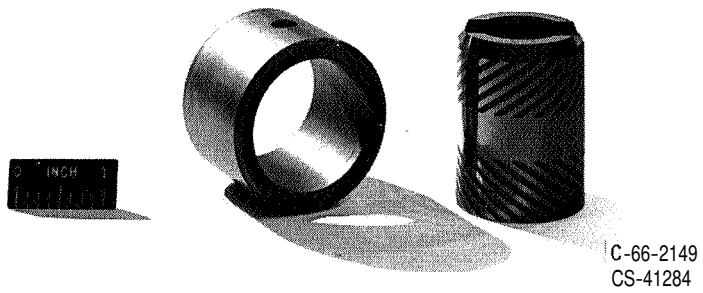
Figure 3. - Plain bearing (MP-3) versus Herringbone groove journal (K-14) after test.
