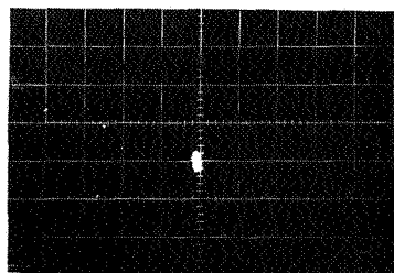
1 CM = 0.5 MILS (A) STABLE OPERATION AT 4100 RPM; 10-LB RADIAL LOAD.
