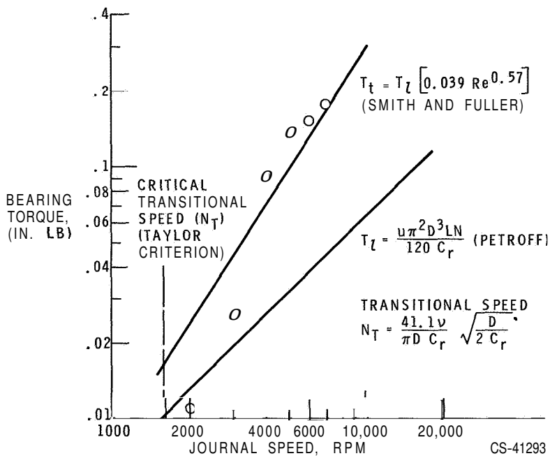
(b) Bearing material, Ni-Cr-Fe-Mo, X; radial clearance, 0.0036 inch; zero load.
