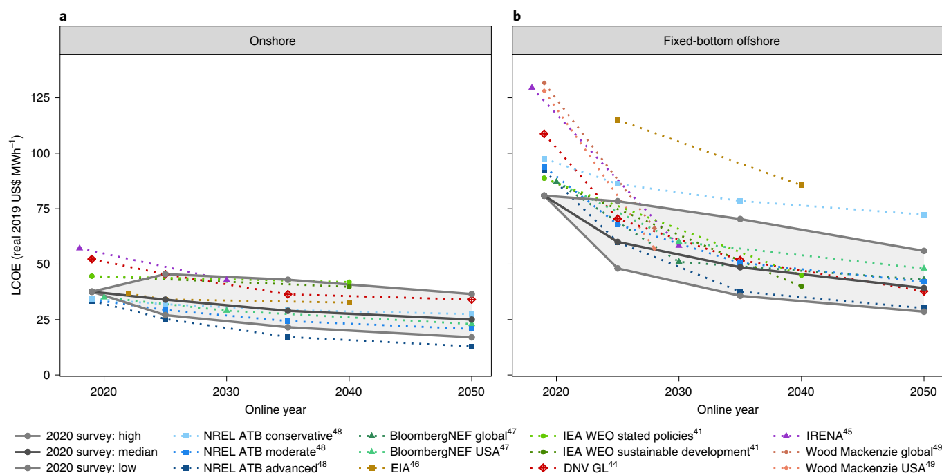
Fig. 8 | Comparison of 2020 survey results with other contemporaneous LCOE forecasts. a,b, Depicts the median of expert responses for LCOE in the median, low and high scenarios for onshore (a) and offshore (b) wind. The shaded areas span the 2020 survey results. Survey results are compared with a range of other LCOE forecasts 41,44–49 . Note that such comparisons are imperfect; for example, some forecasts include offshore transmission-infrastructure costs in LCOE whereas the 2020 survey results exclude those costs. Where possible we apply a geographic weighting across regions to approximate the distribution of the survey respondents. NREL provides a range of cost projections in its Annual Technology Baseline (ATB). The IEA offers two projections in its World Energy Outlook (WEO).
