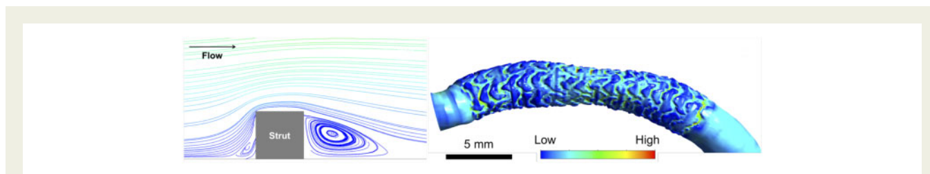
Figure 6 Overview of micro flow environment around a stent strut (left) and the resulting high and low wall shear stress regions around the strut (right).
