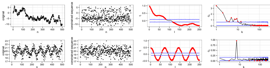
Fig. 2: The sequences in the Toy dataset. The AR (top row) and the periodic sequences (bottom row). Subplots follow the same order as in Fig. 1. The confidence intervals are based on INTERVAL randomization.
