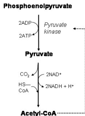
Figure 2: Feedback loop in the linkage between two metabolic systems. In the final reaction of glycolysis, phosphoenolpyruvate produces pyruvate. Pyruvate then produces Acetyl-CoA, some amount of which is needed to continuously replenish the Krebs cycle (not shown). If more Acetyl-CoA is produced than can be used in the Krebs cycle, it accumulates and feeds back (dotted arrow) to inhibit pyruvate kinase, the enzyme responsible for the first step in the reaction.
