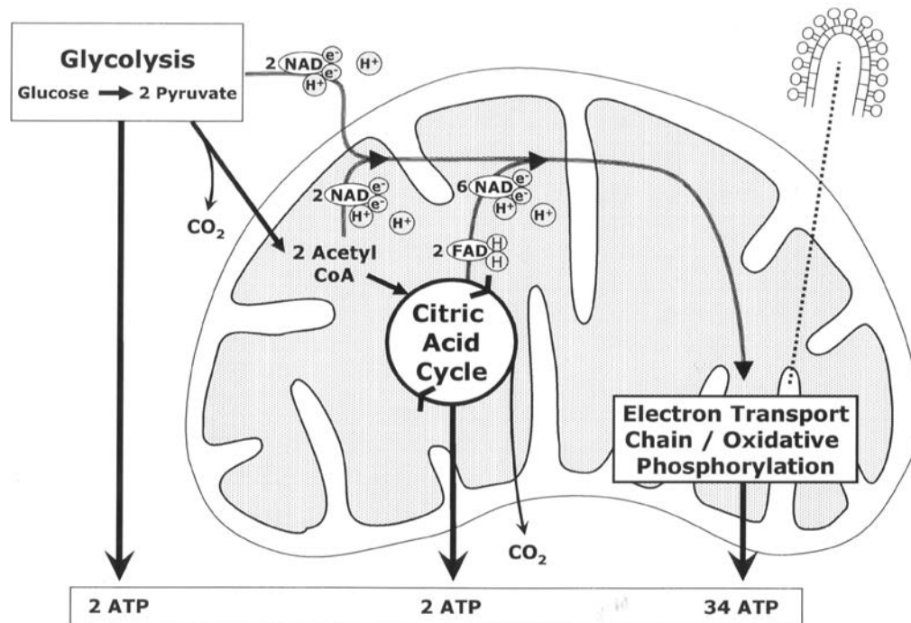
Figure 4: Localization of the three major operations of cellular respiration in parts of the cell: glycolysis in the cytoplasm, the Krebs cycle in the mitochondrial matrix, and the electron transport chain and oxidative phosphorylation in the cristae of the mitochondrion. Also shown is the energy yield from each operation (number of molecules of ATP synthesized from ADP).
