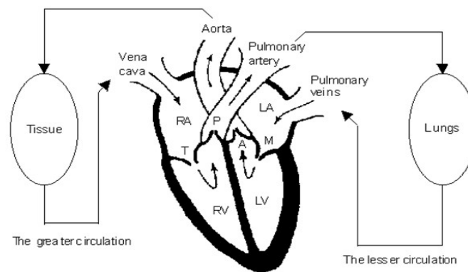
Figure 1. The heart pumping blood. RA: right atrium; LA: left atrium; RV: right ventricle; LV, left ventricle; T: tricuspid valve; M: mitral valve; P: pulmonary valve; A: aortic valve.
