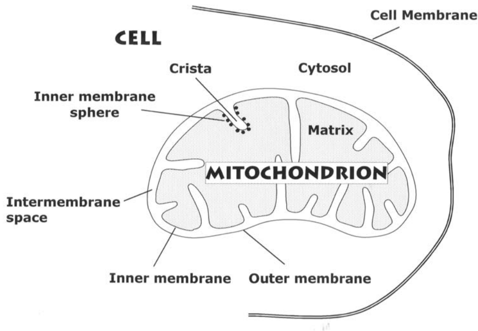
Figure 3: A partial structural decomposition of the cell. The mitochondrion is an organelle located in the cell cytoplasm. The inner membrane of the mitochondrion folds into the inner part (matrix) of the mitochondrion. This creates cristae, on which are located small knobs that contain the enzyme ATPase.
