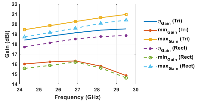
FIGURE 5. Array gain statistical comparison between triangular ( \gamma = 60^\circ ) and square lattice planar array of an array of 8 \times 8 elements as a function of the frequency.
