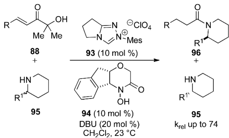
Scheme 22. Kinetic resolution of secondary amines.
