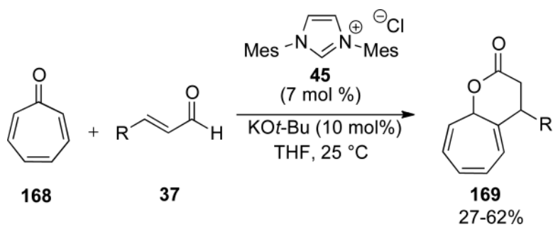
Scheme 48. [8+3] annulation of homoenolate with troponone.
