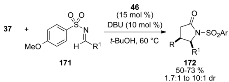
Scheme 49. \gamma -lactam synthesis by homoenolate addition to sulfonylimines.
