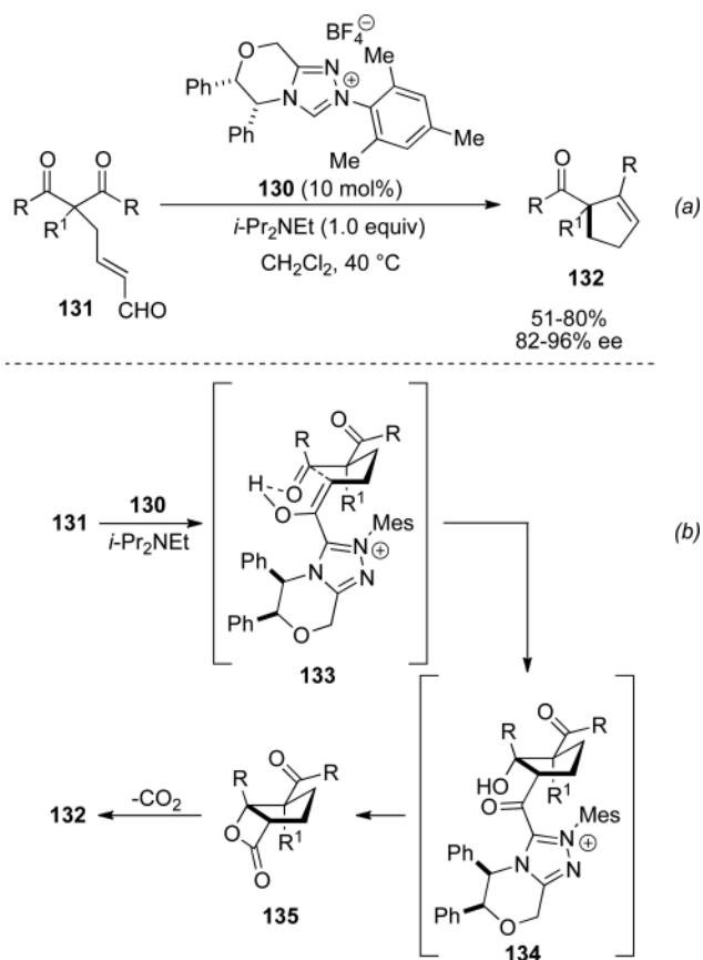
Scheme 38. Decarboxylative cyclization to form cyclopentenes.
