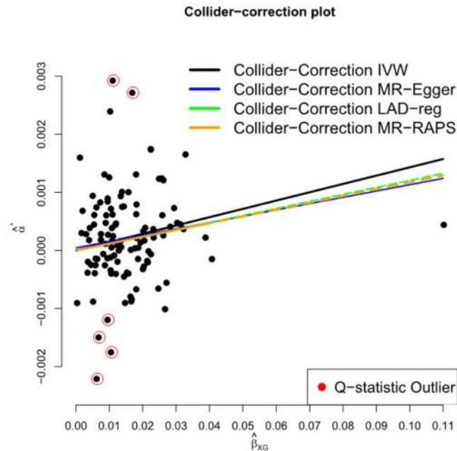
Fig 16. Collider biased SNP outcome associations, \hat{\alpha}_j^* , versus SNP-exposure associations, \hat{\beta}_{XG} for 112 SNPs that were genome-wide significant using 23andMe data only.
