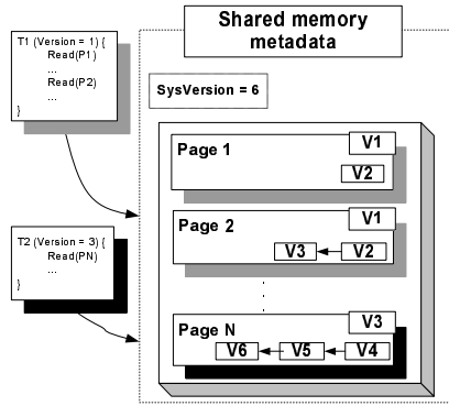
Figure 3. Concurrent “snapshot” creation of disjoint read-set transactions.
