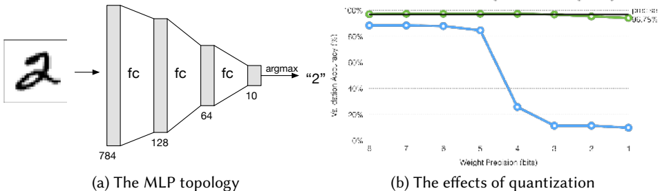
Fig. 3. The multi-layer perceptron (MLP) trained on the MNIST dataset topology and quantization.
