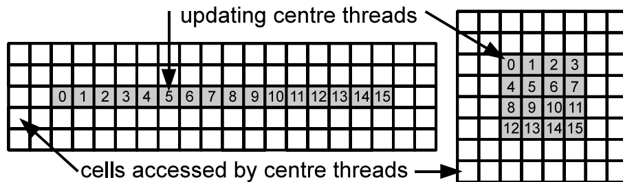
Figure 4: A illustration of two methods of allocating threads to cells within a Cahn-Hilliard field.
