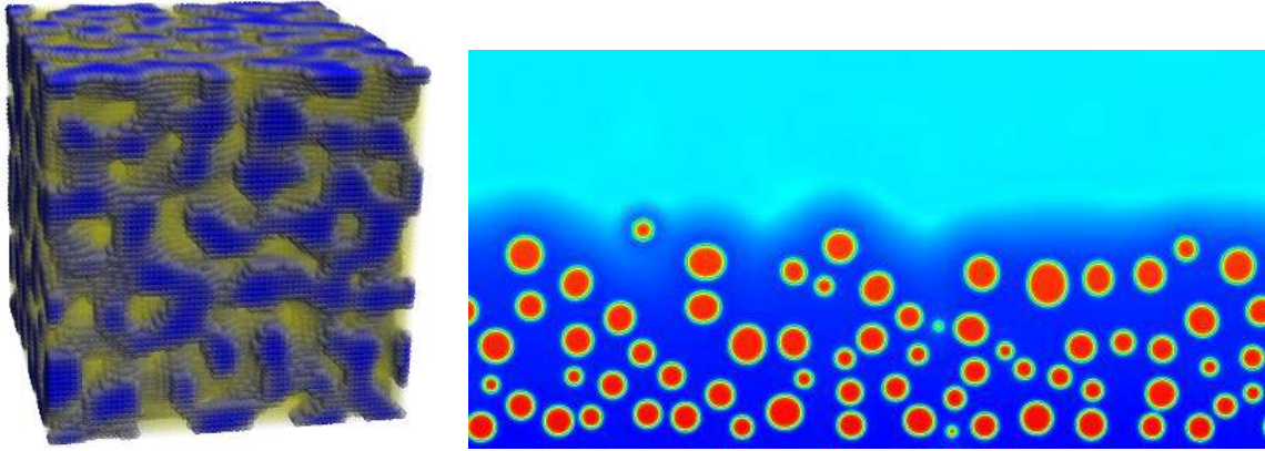
Figure 1: Simulated Cahn-Hilliard systems in: 3-d with a 50/50 symmetric concentration and periodic boundary conditions showing spinodal decomposition (left); and in 2-d with a 25/75 minority concentration showing droplet condensation, with fixed boundary conditions (right).
