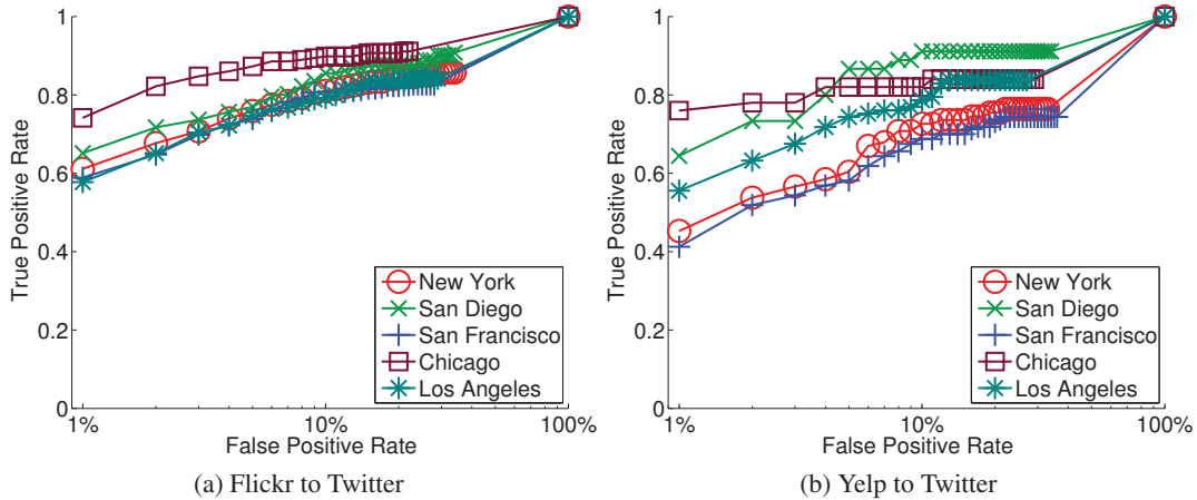
Figure 2: ROC curves for different urban areas for matching Flickr and Yelp users to Twitter users using clusters.
