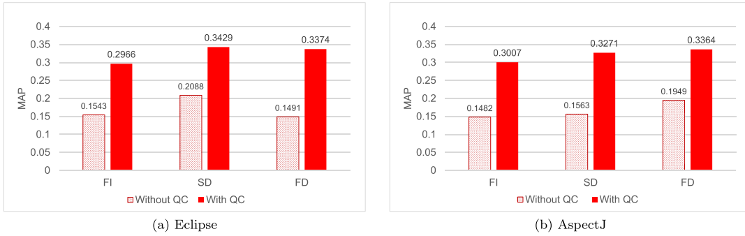
Figure 8. The effect of query conditioning on bug localization with bug reports containing stack traces.
