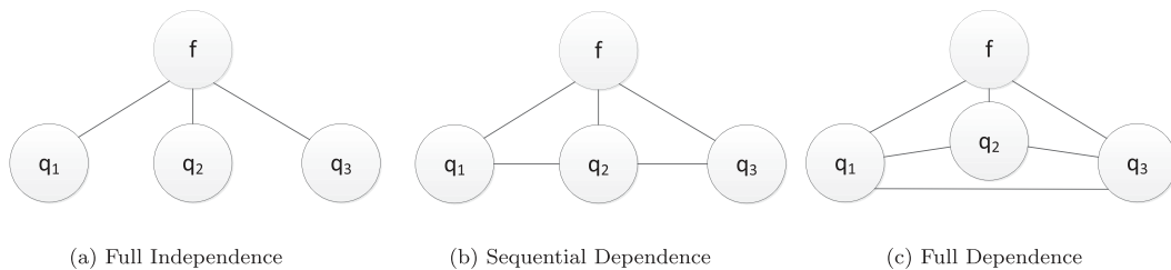
Figure 1. This figure illustrates the notion of a Markov network for capturing the inter-term dependencies in a query vis-à-vis a document. The case depicted is for a query consisting of just three terms. The FI variant shown in (a) corresponds to the Smoothed Unigram Model with retrievals based on Query Likelihoods.
