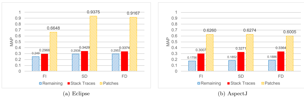
Figure 9. The effect of including structural elements in bug reports on automatic bug localization accuracy. Patches lead to the highest retrieval scores while the bug reports with no stack traces or patches perform the worst in terms of the mean average precision. The number of queries used in these experiments are given in Table III.
