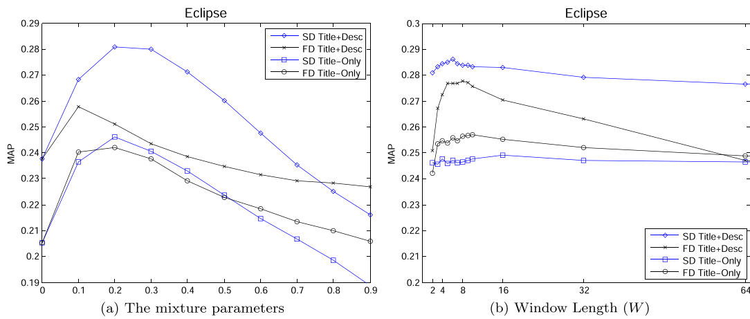
Figure 6. The effects of varying model parameters on mean average precision (MAP) for Eclipse. The figure on the left shows the MAP values as the mixture parameters ( \lambda_{SD} for the sequential dependency assumption and \lambda_{FD} for the full dependency assumption) are varied while the window length parameter is fixed as W = 2 . The figure on the right shows the MAP values as W is varied while the mixture parameters are fixed at 0.2.
