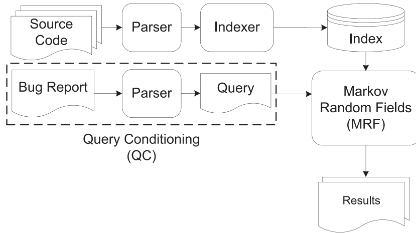
Figure 5. An illustration of the data flow in the proposed retrieval framework.
