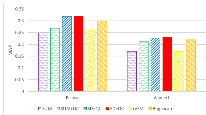
Figure 10. Comparison of the retrieval models for bug localization.
