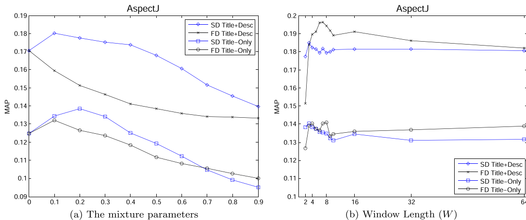
Figure 7. The effects of varying model parameters on mean average precision for AspectJ. The rest of the caption here is the same as for Figure 6.
