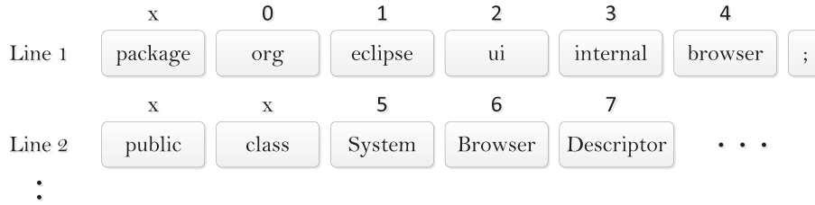
Figure 2. An illustration of indexing the positions of the terms in the Eclipse class SystemBrowserDescriptor.java. The 'x' symbol indicates the stop words that are dropped from the index.
