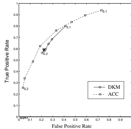
Figure 7: Diabetes Unpruned
