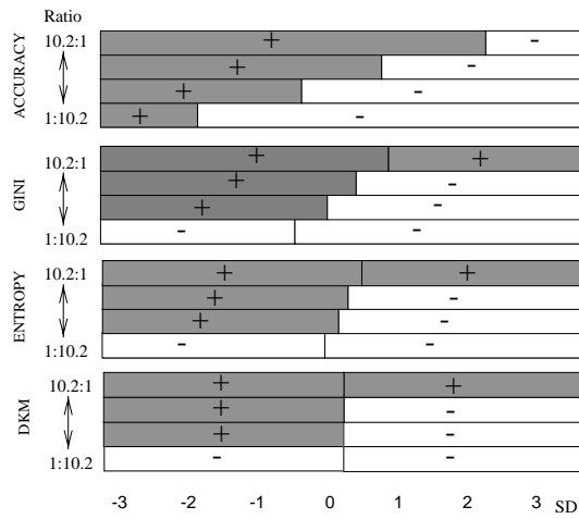
Figure 5: Decision Boundaries
