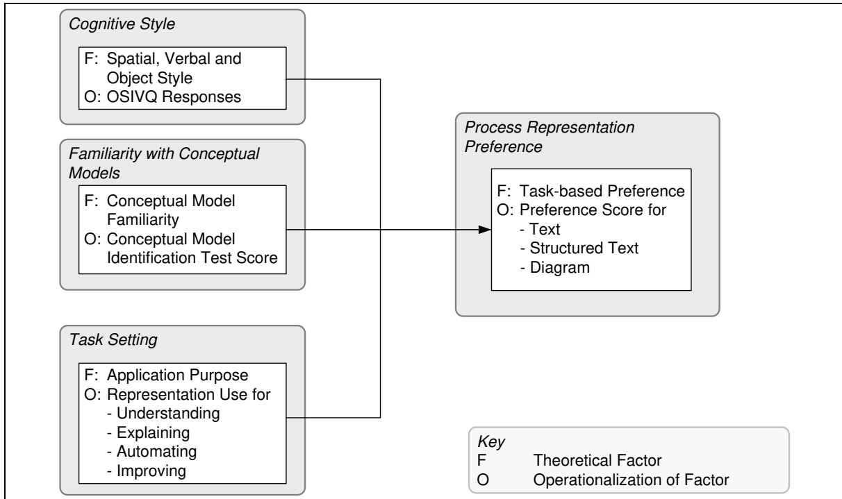
Fig. 2 Research Framework
