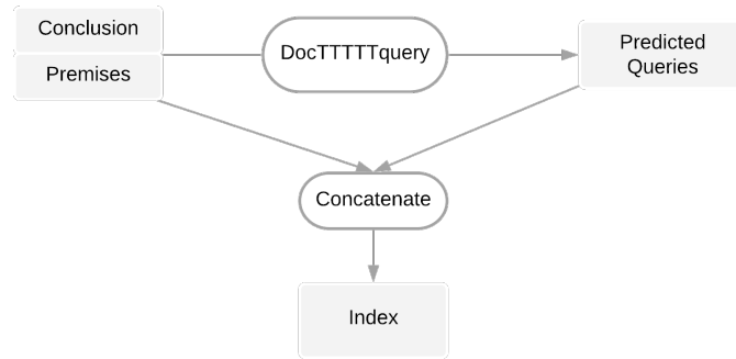
Figure 1: Procedure of document expansion using docTTTTquery
