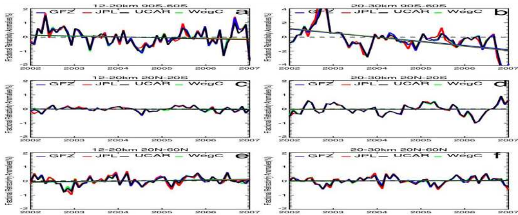
Fig. 32. Comparison of RO data (fractional refractivities) processed by four independent centers, GFZ (GeoForschungsZentrum, Potsdam), JPL, UCAR, and the Wegener Center (WegC) over the period 2002–2007. (a) 12–20 km, 90°–60° S; (b) 20–30 km, 90°–60° S; (c) 12–20 km, 20° N–20° S; (d) 20–30 km, 20° N–20° S; (e) 12–20 km, 20° N–60° N; (f) 20–30 km, 20° N–60° N (Ho et al., 2009c).
