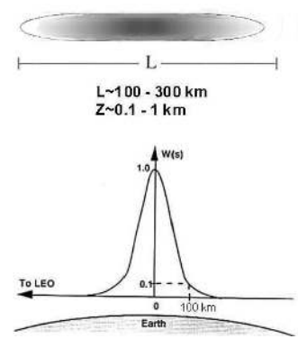
Fig. 3. Top: schematic depiction of tubular volume over which the atmosphere contributes information to a single occultation measurement. The intensity of shading in the tube represents the relative weighting of atmospheric properties that contribute to the value retrieved at the center of the tube. For typical atmospheric structures, L and Z are approximately 300 and 1 km respectively. Bottom: typical along-track weighting function for a single radio occultation measurement (Melbourne et al., 1994). Most of the information is contributed by a mesoscale atmospheric volume centered at the ray tangent point (Anthes et al., 2000).
