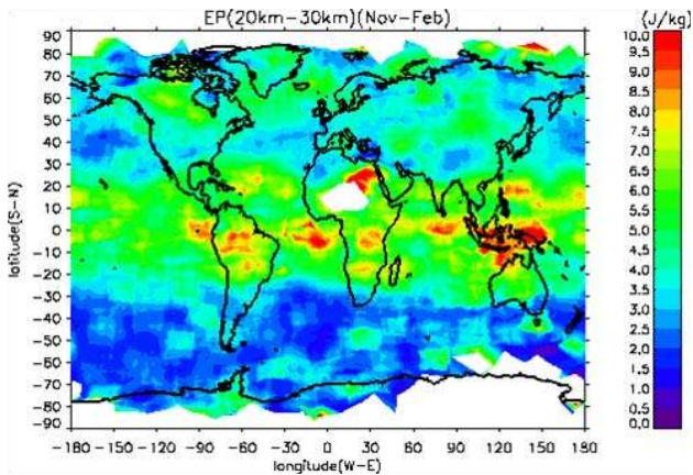
Fig. 11. Gravity wave climatology computed from GPS/MET data during November–February in 1996 and 1997. Colors depict potential energy (EP) between 20 and 30 km for November–February 1996–1997. Warm colors show maximum gravity wave activity as deduced from the GPS/MET vertical temperature profiles. These areas generally coincide with regions of deep convection in the troposphere (Tsuda et al., 2000).
