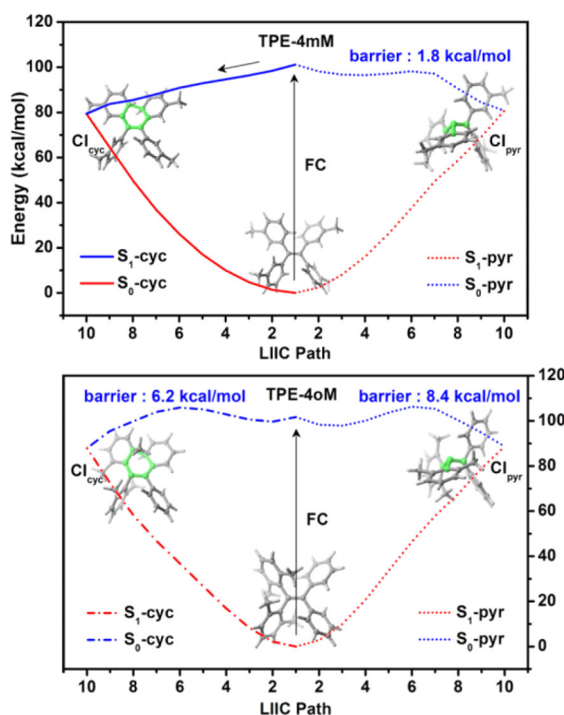
Figure 7. OM2/MRCI-computed LIIC paths connecting the FC points and the S_1/S_0 CI related to the cyclization and photoisomerization of TPE-4mM (upper panel) and TPE-4oM (lower panel). Adapted with permission from Ref. [44] , https://pubs.acs.org/doi/10.1021/acs.jpca.7b00197 . Copyright 2017 American Chemical Society (ACS). Further permissions related to this material should be related to the ACS.
