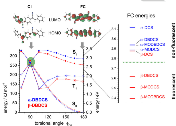
Figure 5. Left panel: TD-DFT rigid torsional scans (S 0 , S 1 and T 1 energies) along a terminal double bond for α-DBDCS and β-DBDCS. Top: CASSCF frontier HOMO- and LUMO-like orbitals characterizing the electronic structure for the CI and FC regions. Right panel: TD-DFT excitation energies calculated at the FC geometry in CHCl 3 . Adapted with permission from Ref. [1]. Copyright 2017 American Chemical Society.
