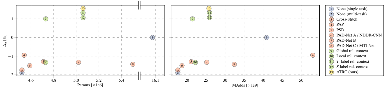
Figure 5. Distillation module resource analysis using an HRNet18 backbone on NYUD-v2. We plot multi-task performance \Delta_m vs. number of parameters (left) and MAdds (right) for multi-task models with different distillation modules inserted before the final prediction layer.
