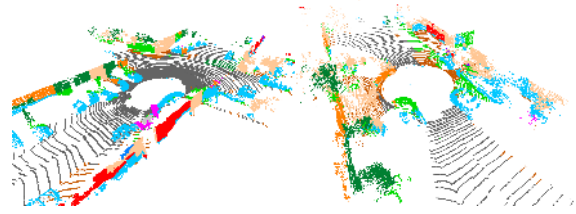
Figure 6: Qualitative results on laser point clouds. Dataset: Velodyne HDL-64E laser scans from KITTI Raw [9]. We trained our model on vKITTI point clouds without color and applied it on real-world laser point clouds. So far, only classes like road, building and car give decent results.
