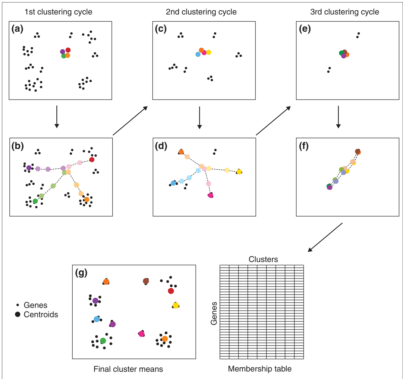
Figure 3 Overview of the FuzzyK method. Genes are represented as points in space, where genes that are similarly expressed are close together. (a) In the first fuzzy-clustering cycle, k/3 centroids are defined as the most informative k/3 eigen vectors identified by PCA of the input dataset (large colored circles). (b) The centroids are refined by iteratively calculating the gene-cluster memberships and updating the centroid positions until convergence (see Figure 2b). (c,d) Genes that are correlated >0.7 to the identified centroids are removed from the dataset, gene and array weights are recalculated, and the entire fuzzy k-means clustering process is repeated on the data subset for an additional k/3 clusters (see Materials and methods for details). (e,f) Steps c and d are repeated for a third round of fuzzy clustering. (g) The output of the algorithm is a list of unique centroids and a table of gene-cluster memberships.
