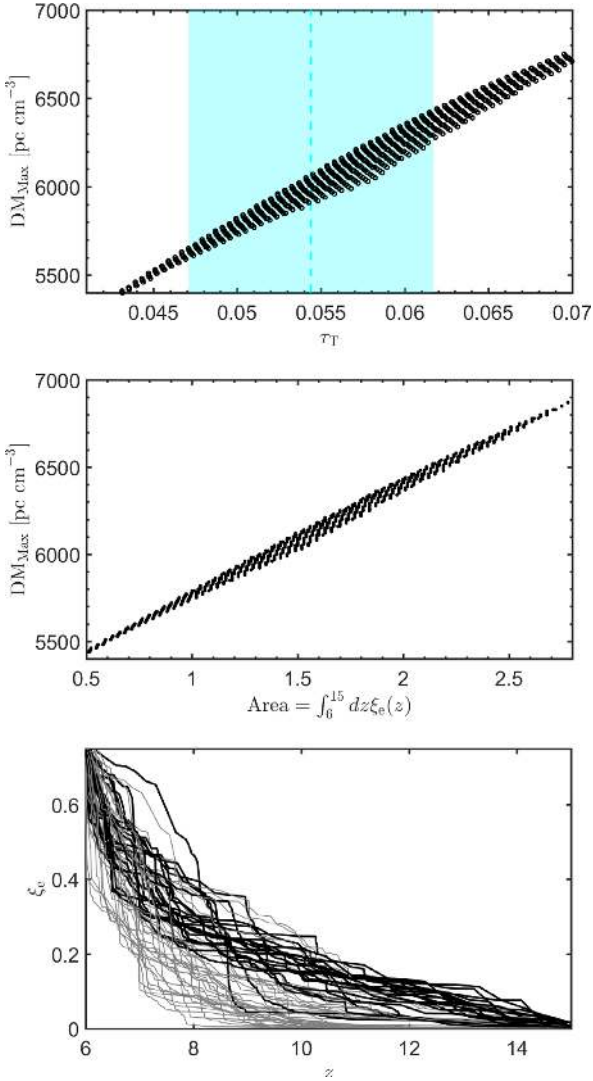
Figure 5. DM_{\max} (IGM contribution) versus Thomson optical depth between us and the last scattering surface, \tau_T , for different H reionization histories (top panel). The correlation between the two suggests that measurement of DM_{\max} can be used to constrain the reionization history, similar to what has previously been done using \tau_T . Reionization histories that give \tau_T = 0.0544 \pm 0.0073 , consistent with Planck measurement (Planck Collaboration 2020) are marked with a cyan shaded region. This panel also shows that if the error in the measurement of DM_{\max} is \lesssim 500 \text{ pc cm}^{-3} then that would provide a more accurate measurement of \tau_T than Planck 2020. The middle panel quantifies the relation between DM_{\max} and reionization history; the X-axis is \int_6^{15} \xi_e(z) dz , i.e. the total area of electron per baryon for 6 < z < 15 . The bottom panel shows examples for \xi_e(z) curves (in grey) that are consistent with the Planck 2020 measurement of \tau_T . Thick black curves are consistent with \tau_T (Planck 2020 data) and with DM_{\max} = 6000 \pm 100 \text{ pccm}^{-3} .
