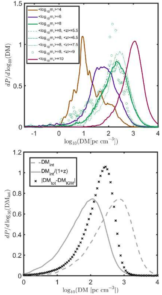
Figure 6. Top: distribution of intrinsic (ISM + CGM) contribution to DM from high-redshift galaxies in the FIRE simulations. Thin lines depict distributions dependent on both galaxy stellar mass (within bins of \Delta \log_{10}(m_*) \pm 0.5 ) and redshift (within bins of \Delta z \pm 0.5 ), while thick lines depict the distributions averaged over redshift (in the range z = 5-12 ), but still dependent on galaxy stellar mass. Bottom: A grey line shows the distribution averaged over both galaxy mass and redshift (integrated over the range of m_* and z explored by the FIRE simulations, \log_{10}(m_*/M_\odot) = 3.5-10.5 and z = 5-12 ), as weighted by the star formation and stellar mass functions accordingly (see Section 3.3 for details). We present both the distribution in the galaxy comoving frame (dot-dashed) and the distribution in the observed frame, in which the DM from a galaxy at z is reduced by a factor of 1+z (solid). The overall distribution of the error in DM_{\text{IGM}}(z) , given by |DM_{\text{tot}} - DM_{\text{IGM}}| weighted by the star formation and galaxy mass functions and integrated over all redshifts and all stellar masses is depicted by black \times s. We stress that these ‘averaged’ distributions shown in the bottom panel are presented for clarity and are not directly used in our Monte Carlo calculation presented in Section 3.5.
