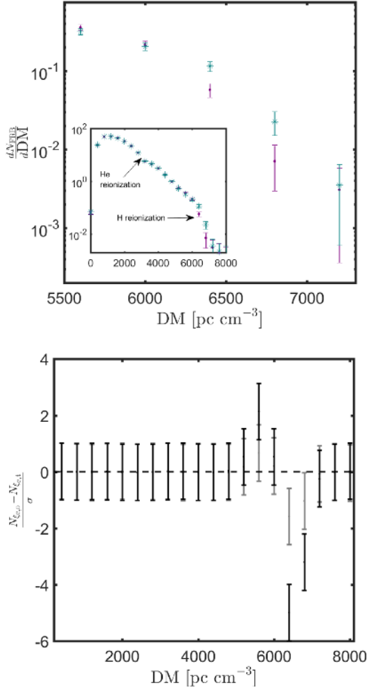
Figure 7. Top: Distribution of dN_{\text{FRB}}/d\text{DM} resulting from a Monte Carlo simulation, with N = 10^5 detected FRBs, grouped in bins of constant width, \Delta\text{DM} = 400 \text{ pccm}^{-3} . The purple (cyan) error bars centred on dots (asterisks) depict 1\sigma fluctuations about the mean value for the ionization fraction as described by \xi_{e,o}(z) (Robertson et al. 2015; \xi_{e,t}(z) defined in equation 5). Bottom: Deviations between the model using \xi_{e,o}(z) relative to \xi_{e,t}(z) (equation 5). The former model results in a relative excess of bursts with 5000 \text{ pccm}^{-3} \lesssim \text{DM} \lesssim 6000 \text{ pccm}^{-3} and a dearth of bursts with 6000 \text{ pccm}^{-3} \lesssim \text{DM} \lesssim 7000 \text{ pccm}^{-3} . The grey bars depict results with N = 10^4 detected bursts and the black with N = 10^5 detected bursts.
