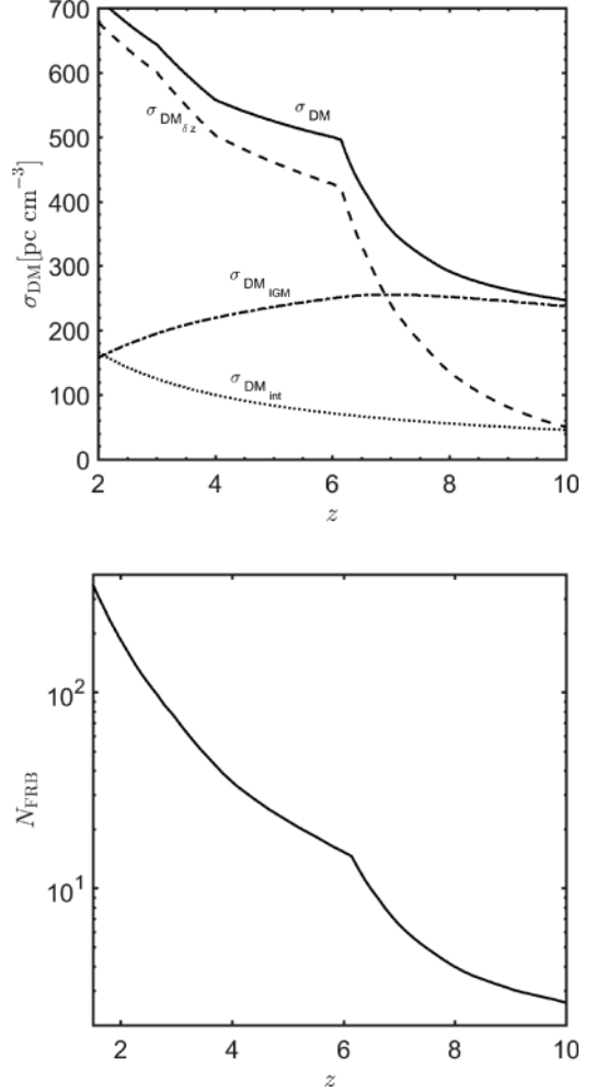
Figure 9. The upper panel shows contributions to \sigma_{\text{DM}} from IGM electron density fluctuations (dash-dot curve marked with \sigma_{\text{DM}_{\text{IGM}}} , using the \xi_{e,o}(z) reionization history), host galaxy+CGM from FIRE simulations (dots, labelled \sigma_{\text{DM}_{\text{int}}} ), due to error associated with FRB host galaxy redshift measurements which is taken to be 0.5 for this calculation, and due to the finite redshift bin-width which we took to be 1.0 (dash-curve, marked as \sigma_{\text{DM}_{\delta z}} , see equation (24) and calculated for \xi_{e,o}(z) ); we have taken \sigma_{\text{DM}_{\text{IGM}}}(z) = 0.13 \text{ DM}_{\text{IGM}}/(1+z)^{1/2} as per the Jaroszynski (2019) analysis of cosmological simulations. The square-root of the squared sum of these contributions is \sigma_{\text{DM}} (solid line). Note that \sigma_{\text{DM}_{\text{int}}} decreases with redshift as (1+z)^{-1} in the observer frame. The lower panel shows the number of FRBs for which redshift should be measured with an accuracy of \Delta z = 0.5 in order to determine \langle \text{DM}_{\text{IGM}} \rangle at the average redshift of these bursts with an accuracy of 2.5 per cent.
