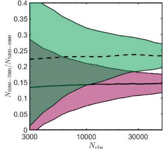
Figure 8. Ratio of detected bursts with 6000 \text{ pccm}^{-3} \lesssim \text{DM} \lesssim 7000 \text{ pccm}^{-3} and those with 5000 \text{ pccm}^{-3} \lesssim \text{DM} \lesssim 6000 \text{ pccm}^{-3} , as a function of the total number of detected bursts, N , for models with different reionization histories [purple region / solid line for \xi_{e,o}(z) (Robertson et al. 2015) and green region / dashed line for \xi_{e,t}(z) defined in equation (5)].
