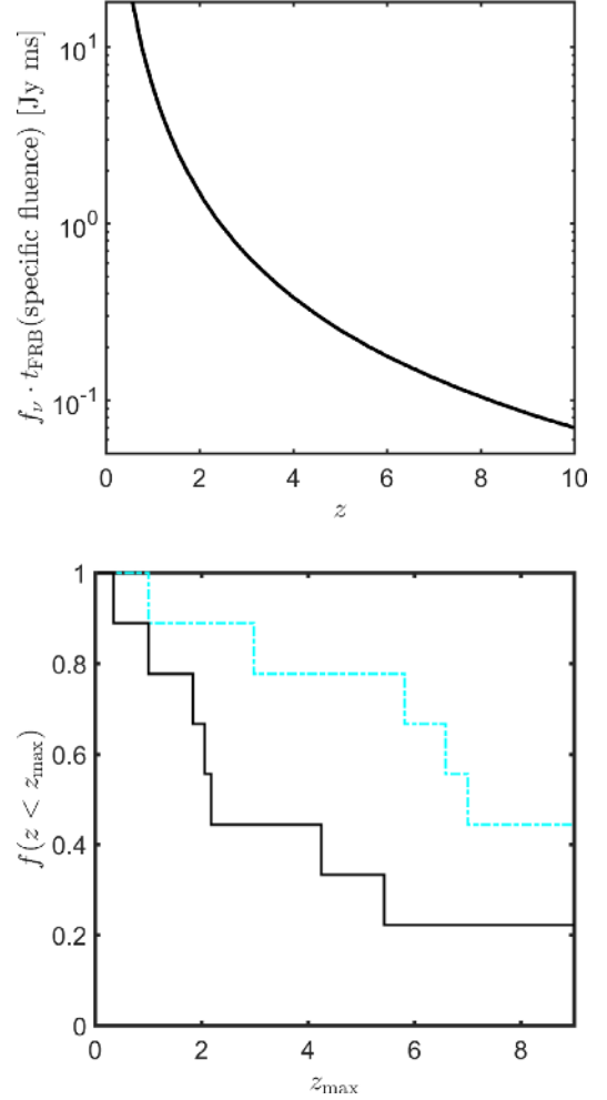
Figure 2. Top: The observed specific fluence ( f_\nu \times t_{\text{FRB}} ) is shown for an FRB at redshift z that has an isotropic equivalent energy per unit frequency of 10^{32} erg Hz ^{-1} at 1.0 GHz in its rest frame. The spectrum of the burst is taken to be L_\nu \propto \nu^{-1.5} , t_{\text{FRB}} is the observed burst duration and the burst is observed at 500 MHz, i.e. \nu in f_\nu is 500 MHz. Bottom: The fraction of nine FRBs with known redshifts which would be detectable up to a redshift z . Results are shown in a solid (dot-dashed) curve for a specific fluence threshold of e_\nu^{\text{th}} = 1 Jy ms ( e_\nu^{\text{th}} = 0.1 Jy ms) at 500 MHz and assuming a spectral slope of \alpha = -1.5 .
