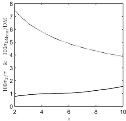
Figure 10. Shown here are \sigma_T/\tau calculated using equation 32 (solid line), and \sigma_{DM_{IGM}}/DM = 0.13/(1+z)^{0.5} (dotted line); both are these are per cent error associated with the fluctuations in the electron density of the IGM.
