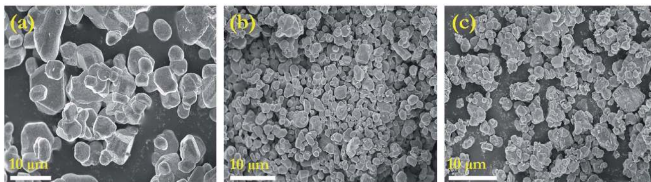
Fig. 3 SEM micrograph of (a) LRO, (b) LRTO and (c) LRFO.
