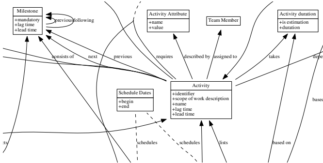
Fig. 3. Fragment of reference model REF visualized as class diagram. Boxes represent entities, arrows relations, and dashed lines link entities to relations.
