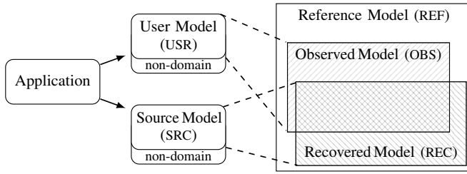
Fig. 1. Domain model recovery for one application.
