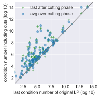
Figure 2: Root node: Comparison of condition numbers of the original LP and including cutting planes.
