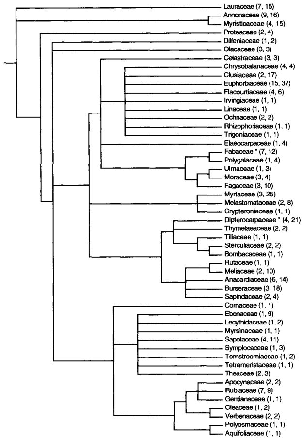
Figure 2: Summary of the composite phylogenetic tree assembled for all the tree taxa in 4.48 ha of rain forest at Gunung Palung. Numbers after family names indicate the number genera and species within that family. An asterisk indicates that published sources (see text) were used to resolve relationships among some genera or species within the family; all other families were modeled as an unresolved polytomy of monophyletic genera, containing unresolved species.
