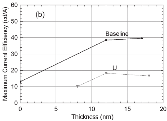
Figure 6. Effect of nucleobase film thickness on maximum observed OLED current efficiency: a) EBL thickness in Type II devices with G, A, and DNA-CTMA compared to Type I (Baseline) Device with NPB EBL; b) HBL thickness in U-based Type II devices compared to Type I (Baseline) Device with BCP EBL.
