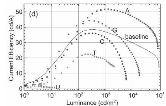
Figure 7. The performance of Type II (NB EBL/HTL) at 17 nm where NB energy levels affect OLED performance: a) current density versus voltage; b) luminance versus voltage; c) luminous efficacy versus current density; and d) current efficiency versus luminance.
