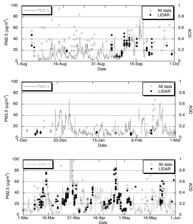
Fig. 2. Time series for PM 2.5 and AOD for the period Aug–Sep (upper panel), Dec–Feb (middle panel) and Mar–May (lower panel). The AERONET L1.5 AOD data are differentiated between data that did (filled diamond) and did not (open diamonds) pass our additional cloud screening based on the LIDAR profiles.
