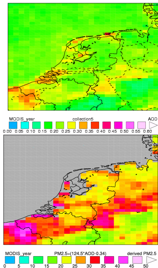
Fig. 11. (a) AOD composite map MODIS and (b) estimated PM 2.5 distribution ( \mu\text{g}/\text{m}^3 ) over the Netherlands and its direct surrounding during situations with predominantly easterly and southerly flow.
