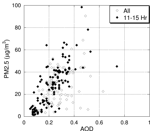
Fig. 9. The variation of PM 2.5 with AOD for all data and those between 11:00 and 15:00 h.
