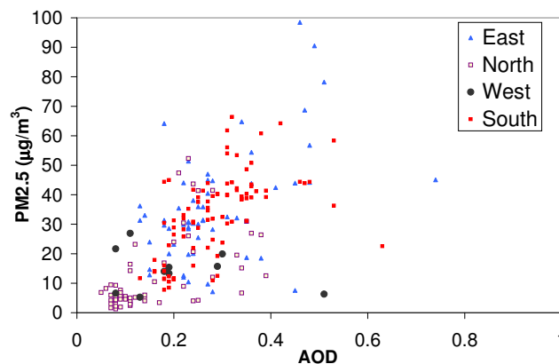
Fig. 8. The variation of PM 2.5 with AOD as function of air mass origin.
