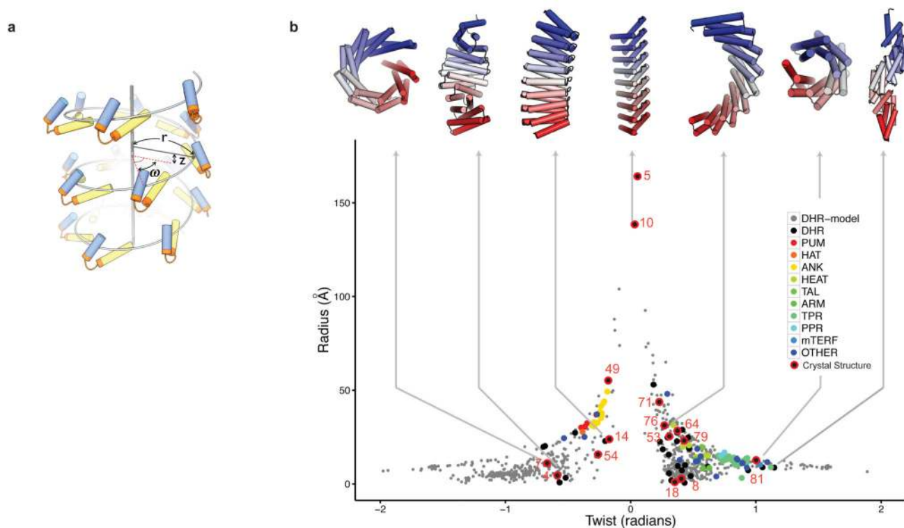
Figure 2. The helical repeat protein universe
