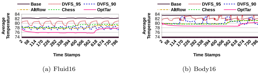
Fig. 21. Snapshot of temporal changes in average chip temperature during a r.
