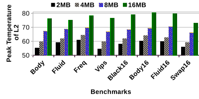
Fig. 4. Size vs LLC's Peak Temperature (in °C).
