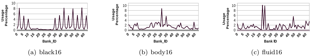
Fig. 7. Non uniform distribution of cache bank accesses.
