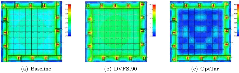
Fig. 22. On-chip spatial thermal behaviour generated by Hotspot 6.0 [46] for Fluid16 at some certain instance during r. Temperature Ranges for three configurations-(a) Baseline: 336K to 364K, (b) DVFS_90: 334K to 360K, (c) OptTar: 332K to 358K. Red colour represents peak value where Blue represents the lowest temperature.
