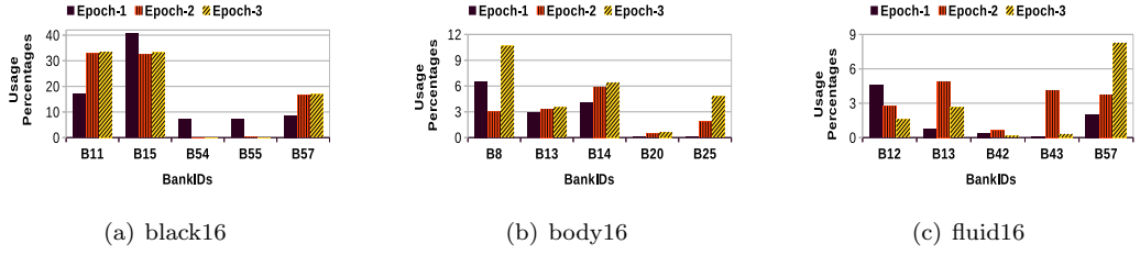
Fig. 8. Change in cache bank access behaviour over time.
