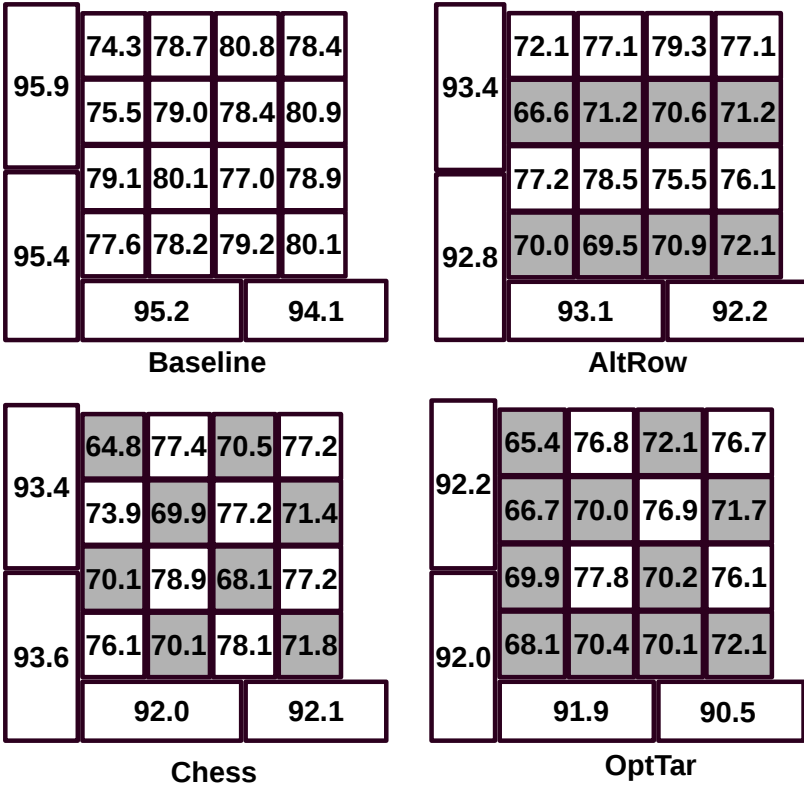
Fig. 19. Temperatures (in ^{\circ}\text{C} ) of the individual banks during r , for Fluid16.
