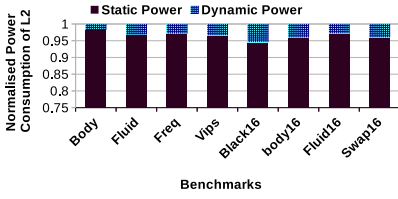
Fig. 3. L2 Power Values: Dynamic and Static.
