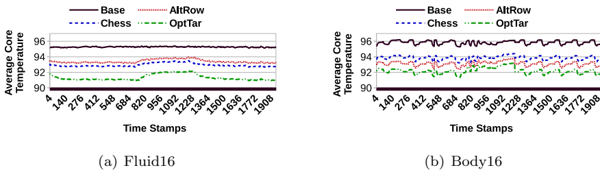
Fig. 18. Snapshot of temporal changes in average temperature of the cores during execution.
