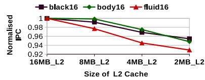
Fig. 6. Change in (Normalised) IPC with respect to Size of LLC.
