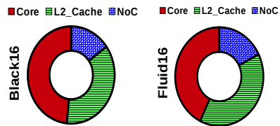
Fig. 2. Percentage contributions of the major on-chip components to the total on-chip power consumption. All values include both Dynamic & Static power (for Black16 & Fluid16).
