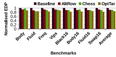
Fig. 14. EDP Savings of the chip.
