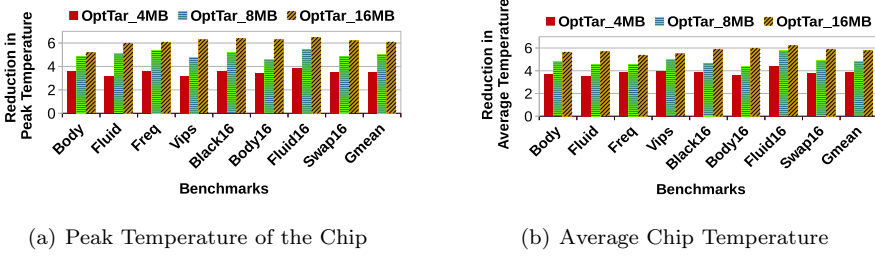
Fig. 23. Comparing temperature reduction (in °C) with different cache sizes.
