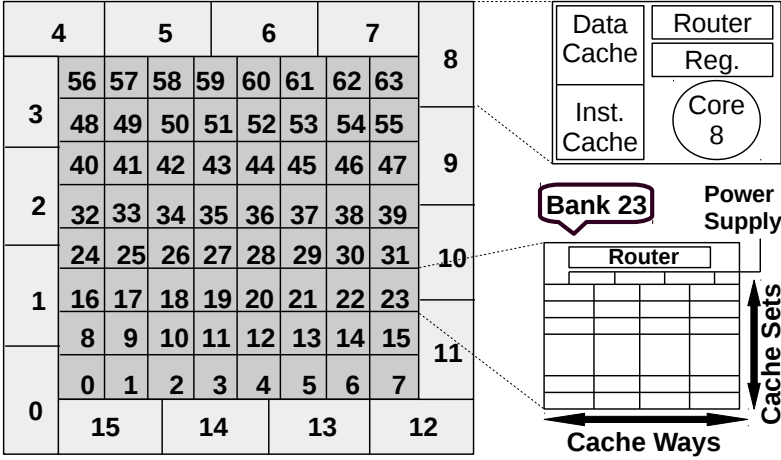
Fig. 9. Internals of our baseline CMP.
