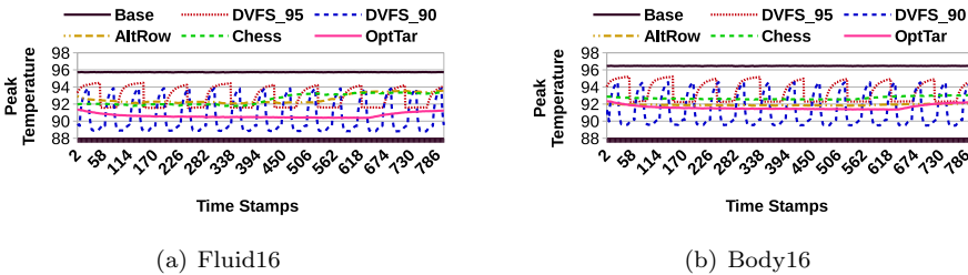
Fig. 20. Snapshot of temporal changes in peak chip temperature during a r .
