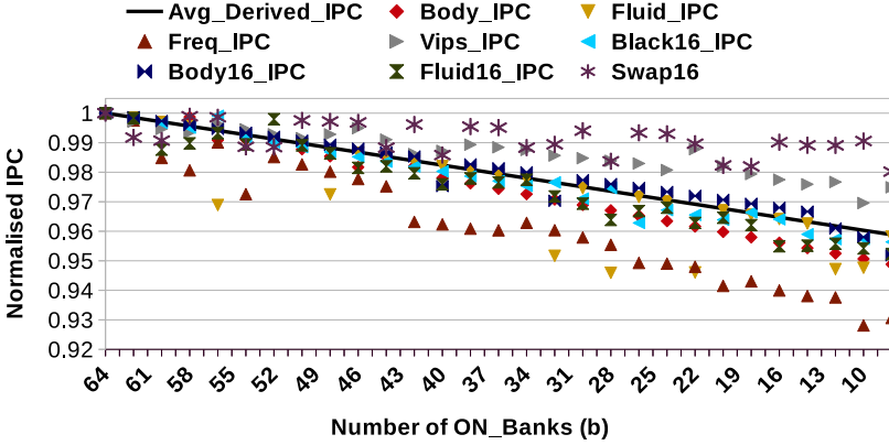
Fig. 10. Relationship between IPC and Cache Size.
