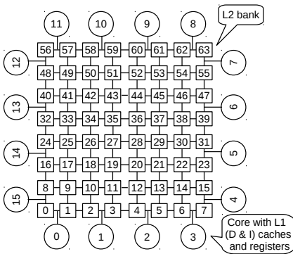
Fig. 1. Baseline CMP architecture with multi-banked centralised NUCA L2 as LLC.
