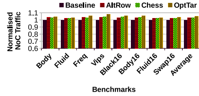
Fig. 16. Increment in NoC Traffic.
