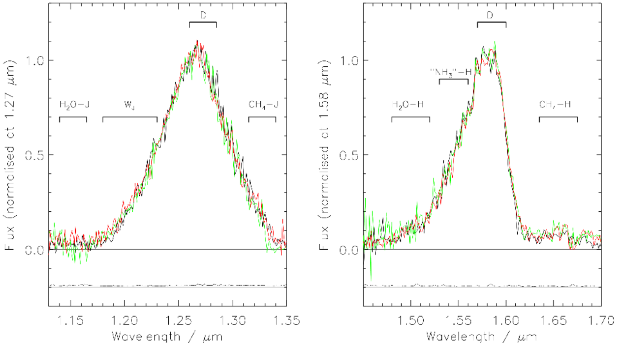
Figure 5. The J and H -band flux peaks of ULAS1335 (black line), ULAS0034 (T9, see text; green line) and CFBDS0059 (T9, see text; red line). The black line that is plotted offset by -0.2 in the y-axis is the error spectrum for ULAS1335. Also indicated are the spectral regions integrated to form the numerator of the spectral indices discussed in the text. The region that forms the denominator is indicated with the letter “D”.
