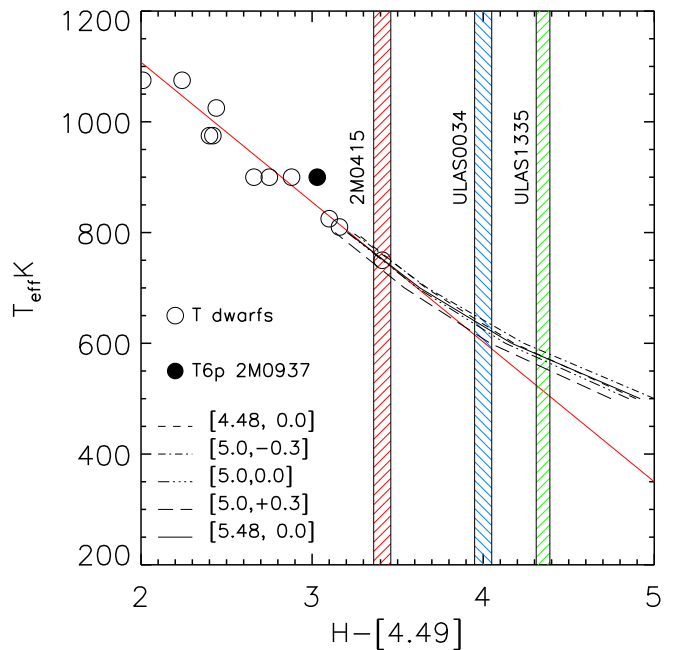
Figure 15. The T_{\text{eff}} - H-[4.49] relation for T dwarfs as defined by Warren et al. (2007). The shaded regions indicate the colours ( \pm 1\sigma ) for the coolest T dwarfs with IRAC magnitudes. The straight red line indicates the empirical fit the colours of warmer T dwarfs. Also plotted, as black lines are theoretical tracks from Marley et al. (2002) and Marley & Saumon (2008). Values for \log g and metallicity are indicated in brackets.
