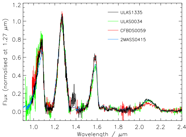
Figure 6. The full YJHK comparison of ULAS1335 to ULAS0034, CFBDS0059 and 2MASS0415.
