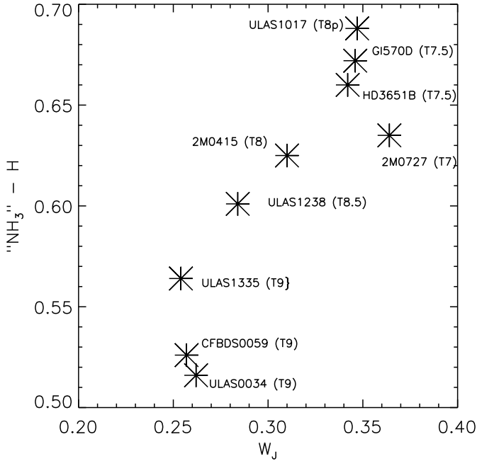
Figure 8. The “NH 3 ”– H index versus W_J index. Uncertainties are not displayed as they are smaller than the symbol size.
