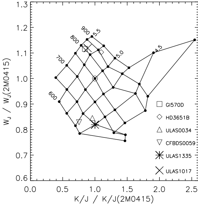
Figure 10. W_J versus K/J indices for a grid of solar metallicity BT-Settl model spectra. The grid has been normalised by matching the T_{\text{eff}} = 750\text{K} , \log g = 5.0 model indices to the empirical index values for 2MASS0415, which lies at (1.0, 1.0).
