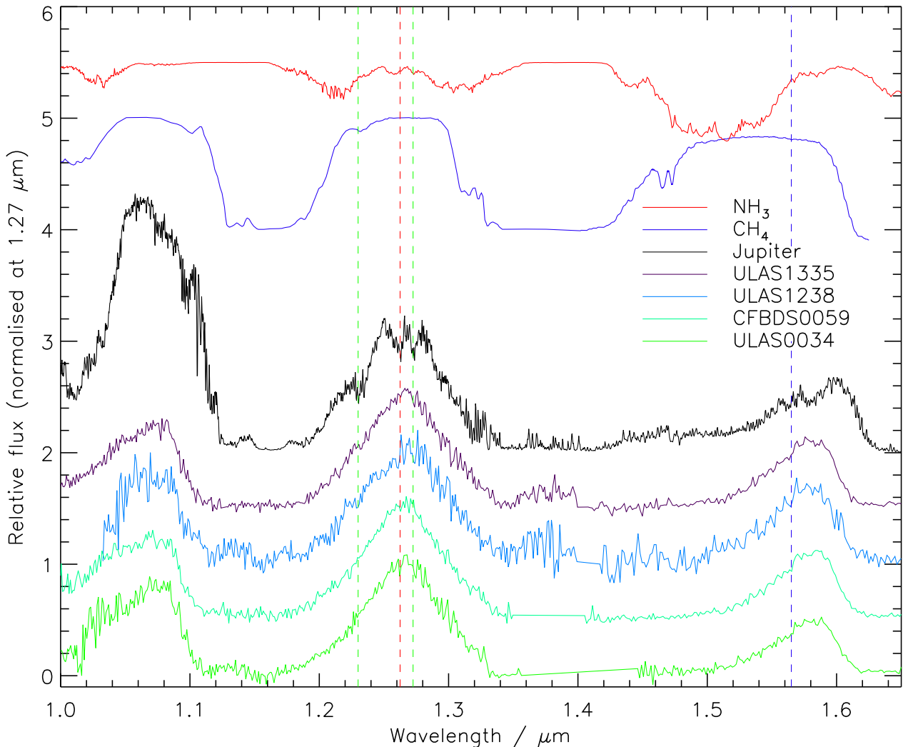
Figure 16. Spectra for ULAS0034, CFBDS0059, ULAS1238 and ULAS1335 compared with the near-infrared spectrum of Jupiter (J. T. Rayner, M. C. Cushing, & W. D. Vacca 2008, in preparation) and laboratory transmission spectra of methane (Cruikshank & Binder 1969) and ammonia (Irwin et al. 1999). The vertical green dashed lines highlight narrow features that appear to be common to ULAS1238, ULAS1335 and Jupiter. The vertical red dashed line highlights an interesting feature in the Jovian spectrum that is absent from the T dwarf spectra (see text). The vertical blue dotted line indicates the location of the red edge of the broad absorption attributed to ammonia by Delorme et al. (2008).
