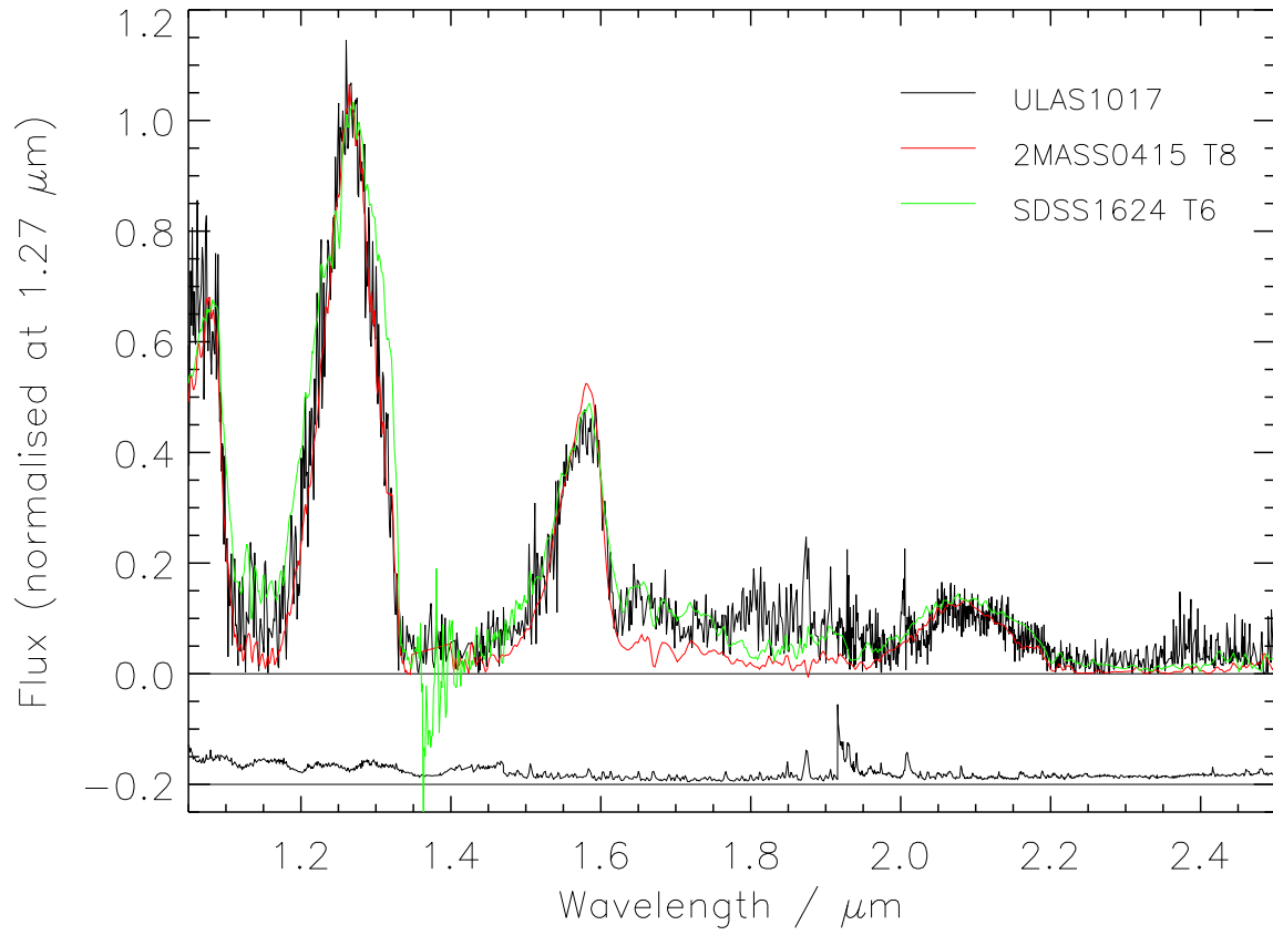
Figure 3. The IRCS+NIRI JHK spectrum of ULAS1017 (black line) overlaid with the spectra of the T8 standard 2MASS0415 and the T6 standard SDSS1624. The error spectrum, offset by -0.2 in the y-axis, is plotted as a black line.
