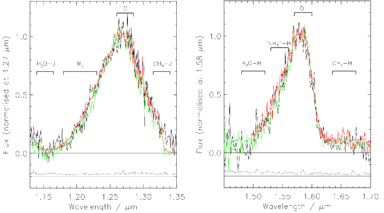
Figure 4. The J and H -band flux peaks of ULAS1238 (black line), ULAS0034 (T9, see text; green line) and 2MASS0415 (T8; red line). The black line that is plotted offset by -0.2 in the y-axis is the error spectrum for ULAS1238. Also indicated are the spectral regions integrated to form the numerator of the spectral indices discussed in the text. The region that forms the denominator is indicated with the letter “D”.
