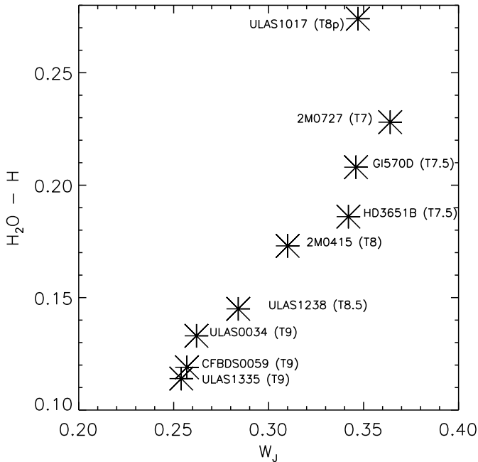
Figure 9. The H 2 O– H index versus W_J index. Uncertainties are not displayed as they are smaller than the symbol size.
