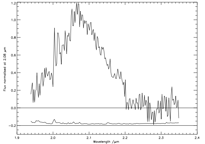
Figure 2. The NIRI K -band spectrum for ULAS1238. The error spectrum is shown offset by -0.2.
