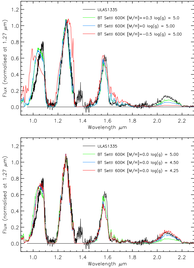
Figure 13. A comparison of model spectra with ULAS1335 for differing gravity and metallicity combinations at T_{\text{eff}} = 600\text{K} .
