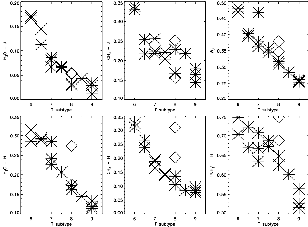
Figure 7. Spectral index versus T-subtype for T6-T9 dwarfs. Asterisks indicate “normal” dwarfs, whilst the diamonds indicate two T8p dwarfs: ULAS1017 and 2MASS J07290002-3954043. Index values for these objects are drawn from Burgasser et al. (2006), Warren et al. (2007), Delorme et al. (2008) and Looper et al. (2007), or are calculated from the objects’ spectra supplied by these authors. Uncertainties are smaller than the symbol sizes.
