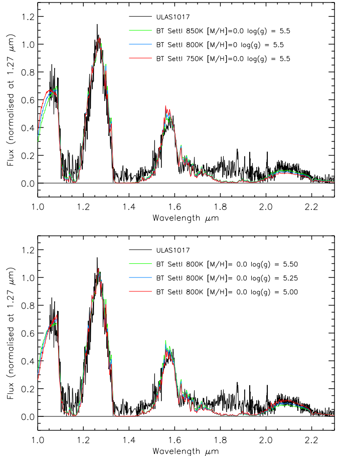
Figure 11. A comparison of model spectra for the parameters bracketing the location of ULAS1017 in the solar metallicity (W_J, K/J) plane.
