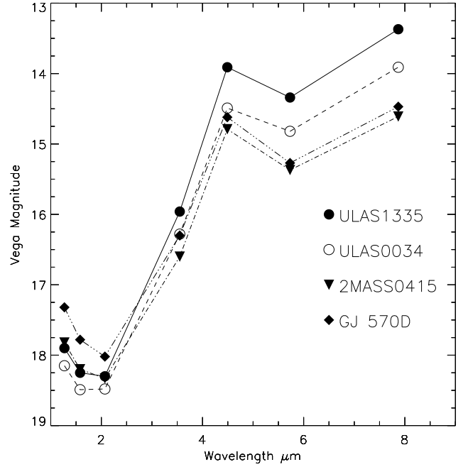
Figure 14. The 1-8 \mu\text{m} SEDs for ULAS1335, ULAS0034 (Warren et al. 2007), 2MASS0415 and GJ 570D. The photometry for the latter two objects, taken from Leggett et al. (2002) and Patten et al. (2006), has been offset by +2.5 magnitudes to allow comparison with the T8+ dwarfs. Uncertainties are of comparable size to the symbols.
