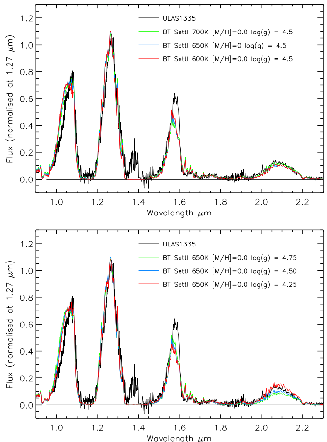
Figure 12. A comparison of model spectra for parameters bracketing the location of ULAS1335 in the solar metallicity (W_J, K/J) plane.
