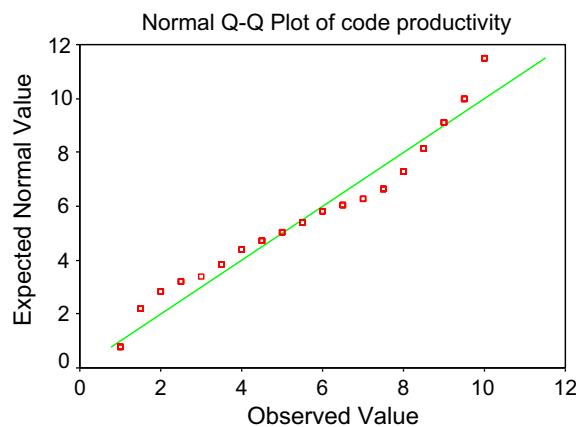
Fig. 4. Code productivity Q-Q graph.
