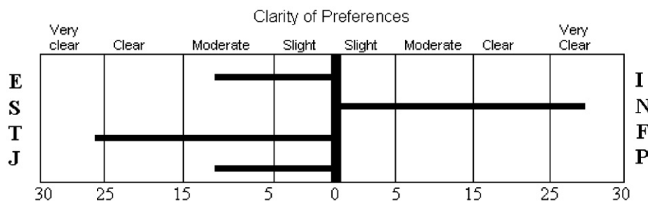
Fig. 1. The strengths of MBTI type preferences.
