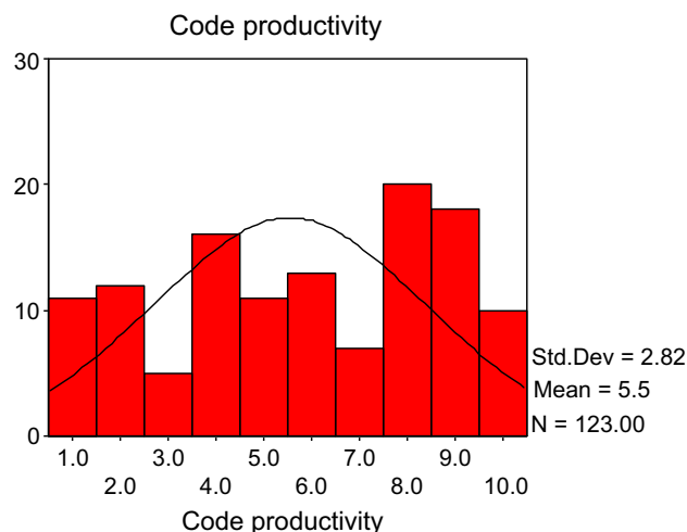
Fig. 3. Code productivity histogram.
