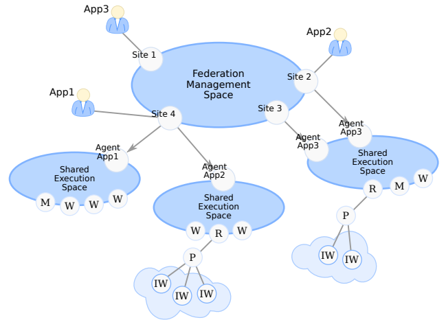
Figure 2: Architecture of CometCloud-based federation model. Here, (M) denotes a master, (W) is a worker, (IW) an isolated worker, (P) a proxy, and (R) is a request handler. Arrows represent deployment of a computational site, while lines show communication.
