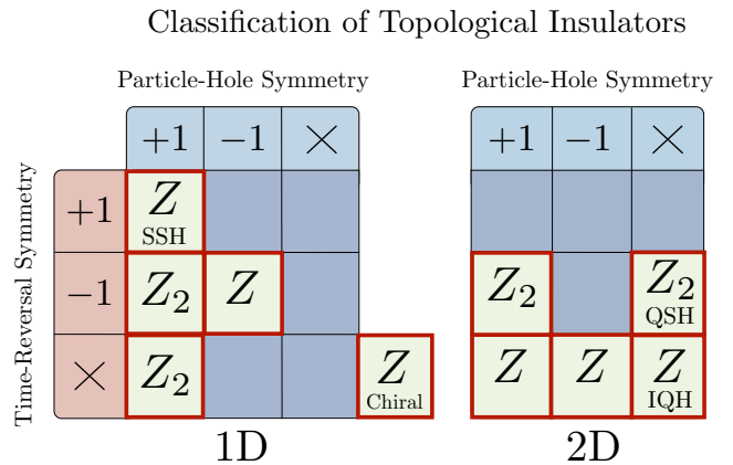
FIG. 1: Classification of topological phases by symmetry for one (1D) and two (2D) dimensions, adapted from Ref.[26, 27]. Discrete time quantum walks can naturally realize all ten classes of nontrivial topological phases in 1D and 2D. Time reversal symmetry (TRS) and particle-hole symmetry (PHS) are defined by the existence of antiunitary operators \mathcal{T} and \mathcal{P} satisfying Eqs.(7) and (8), and may be absent, or present with \mathcal{T}^2 = \pm 1 ( \mathcal{P}^2 = \pm 1 ). In the absence of both TRS and PHS, a distinct “chiral” symmetry with a unitary \Gamma satisfying Eq.(9) may be found. In each case, the symmetry-allowed phases are classified by an integer ( Z ) or binary ( Z_2 ) topological invariant. Classes containing the Su-Schrieffer-Heeger model (SSH)[15], integer quantized Hall (IQH)[17, 18], and quantum spin-Hall (QSH)[19–23] phases are indicated.
