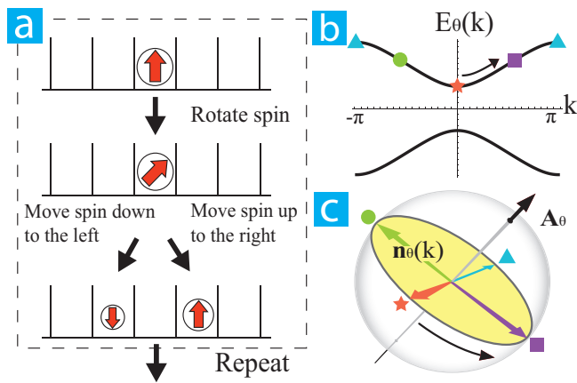
FIG. 2: (a) One dimensional discrete time quantum walk (DTQW) protocol. First, the walker’s internal “spin” is rotated through an angle \theta about the y -axis. Then, the walker is coherently translated by one lattice site to the right (left) if its spin is up (down). The quantum walk is produced by repeatedly applying this combined “step” operation. (b) Band structure of 1D DTQW with \theta = \pi/2 . The spinor eigenstates at each momentum k are directed along the unit vector \mathbf{n}_\theta(k) [see Eq.(6)], as represented on the Bloch sphere in panel (c). Corresponding points in panels (b) and (c) are indicated by the colored markers. For any \theta \neq 0, 2\pi , \mathbf{n}_\theta(k) winds around the origin once as k traverses the Brillouin zone (black arrow). The vector \mathbf{A}_\theta is normal to the plane containing \mathbf{n}_\theta(k) , and defines the axis for the chiral symmetry \Gamma_\theta , see Eq.(9).
