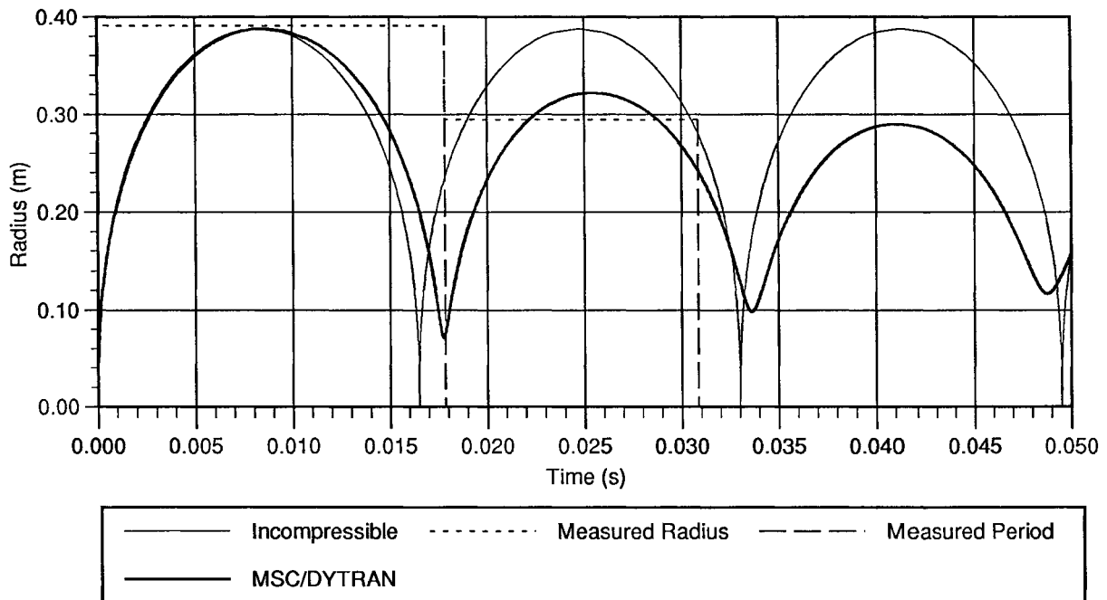
FIGURE 5 Radius versus time behavior for the spherical bubble problem.
