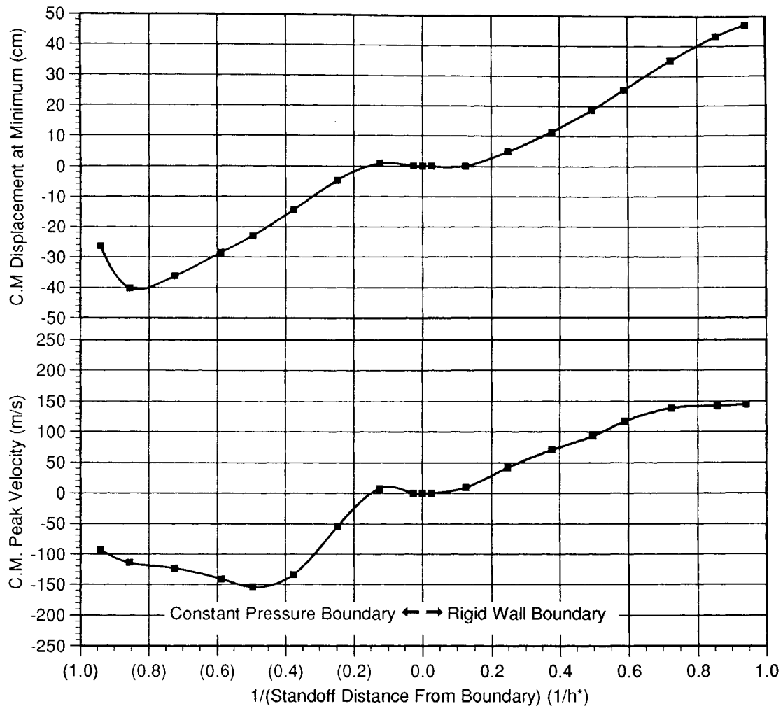
FIGURE 9 Bubble displacement at the first minimum and peak velocity versus the inverse stand-off distance from the boundary (nondimensionalized) for the bubble near the boundary problem.
