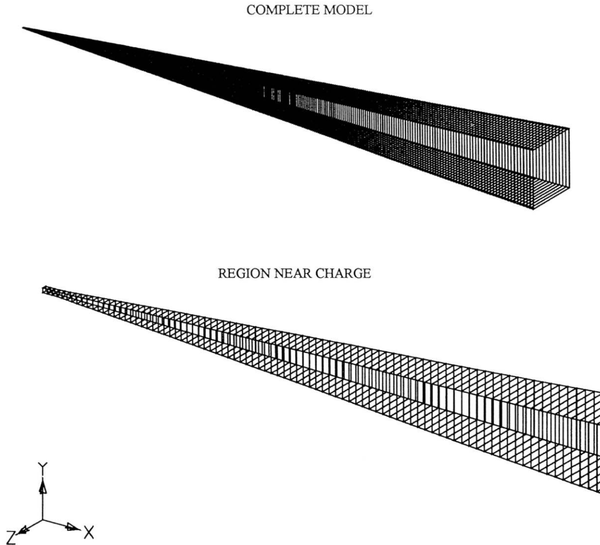
FIGURE 3 Finite element model for the spherical bubble problem.
