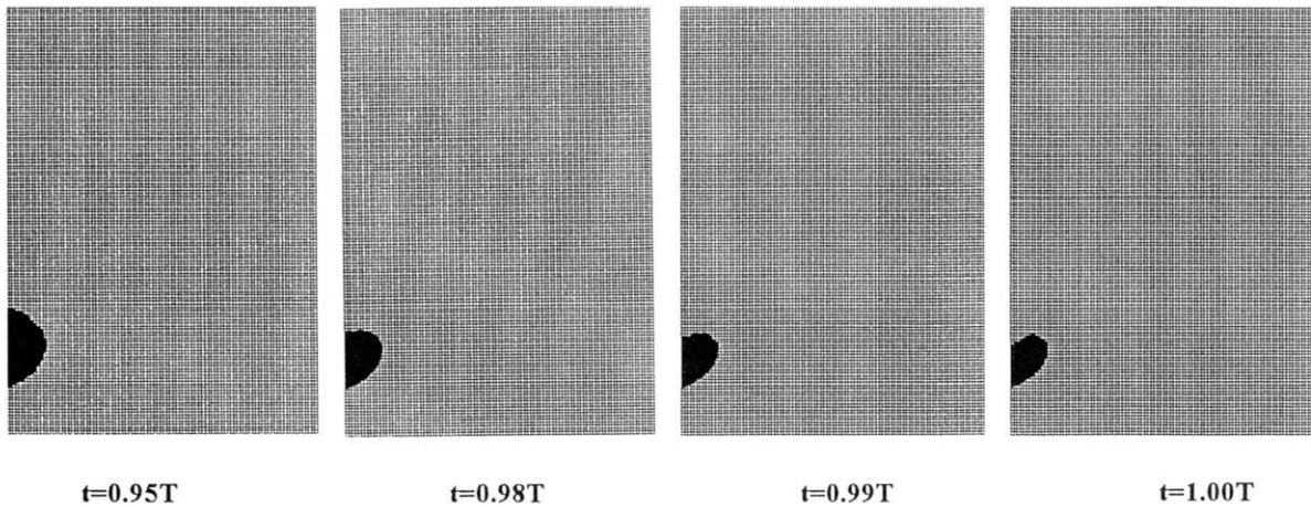
FIGURE 12 Bubble shapes during the final collapse of the bubble at h^* = 1.380 from a rigid wall for the bubble near the boundary problem (boundary located at the bottom).
