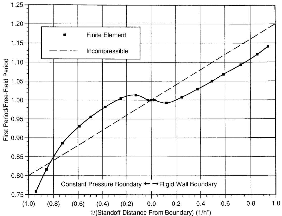
FIGURE 8 Boundary surface effect on the first bubble period versus the inverse stand-off distance from the boundary (nondimensionalized) for the bubble near the boundary problem.
