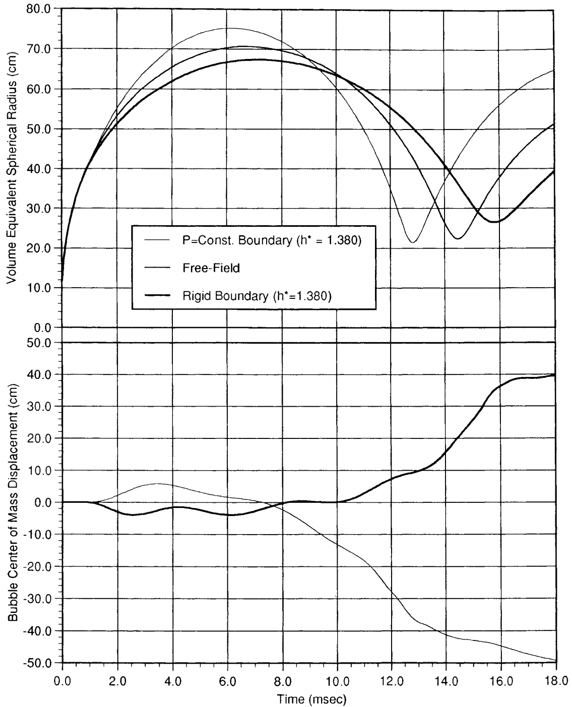
FIGURE 7 Equivalent spherical radius and center of mass displacement versus time behavior for the bubble near the boundary problem (typical).
