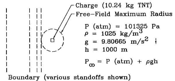
FIGURE 2 Problem geometry for the bubble near the boundary problem.
