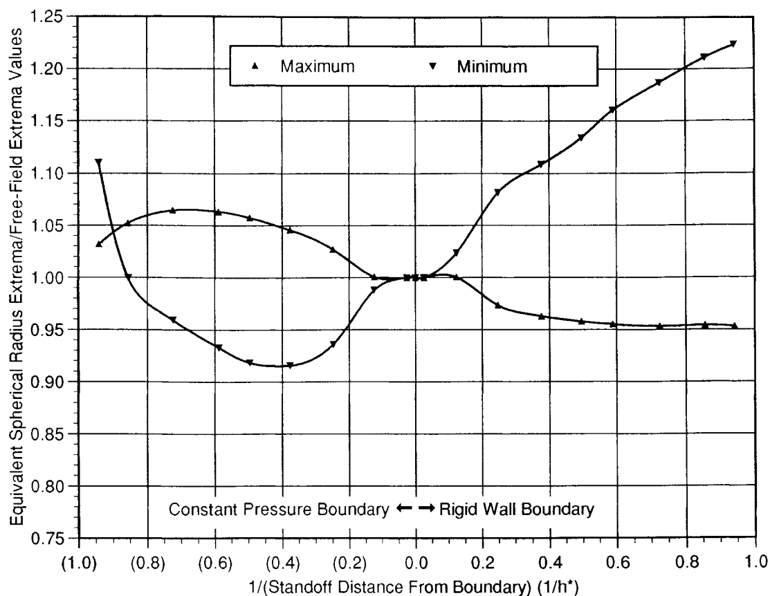
FIGURE 10 Equivalent spherical radius extrema versus the inverse stand-off distance to the boundary (nondimensionalized) for the bubble near the boundary problem.
