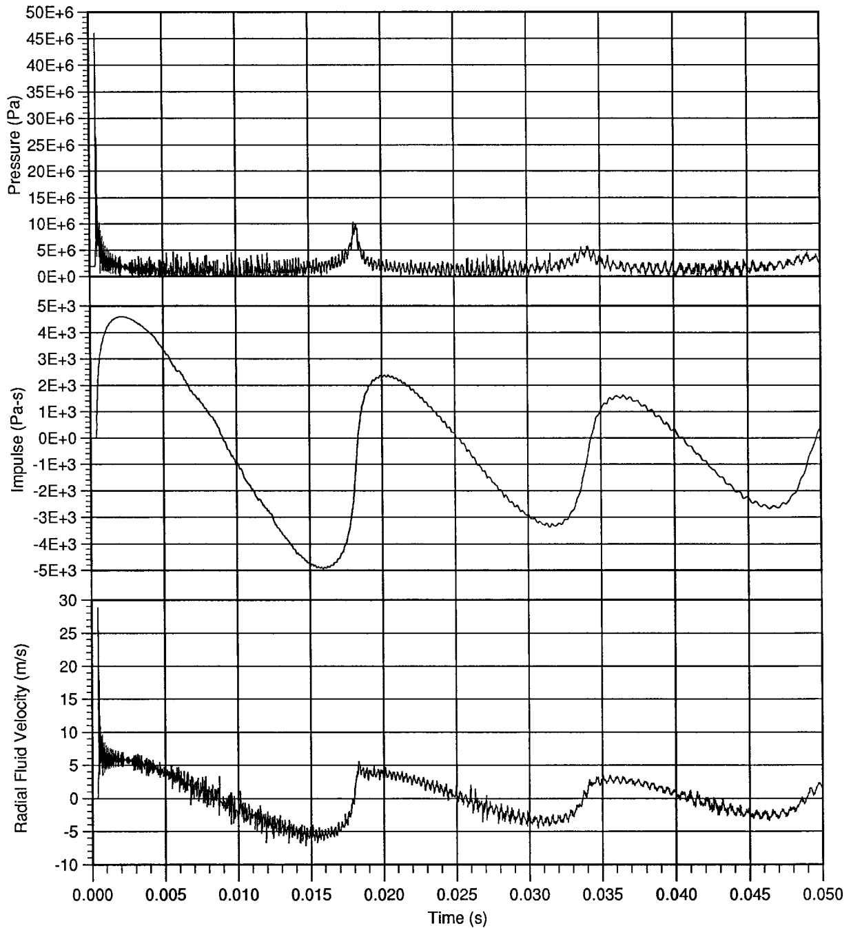
FIGURE 6 Pressure, impulse, and fluid velocity at a point two maximum free-field radii from the charge center for the spherical bubble problem.
