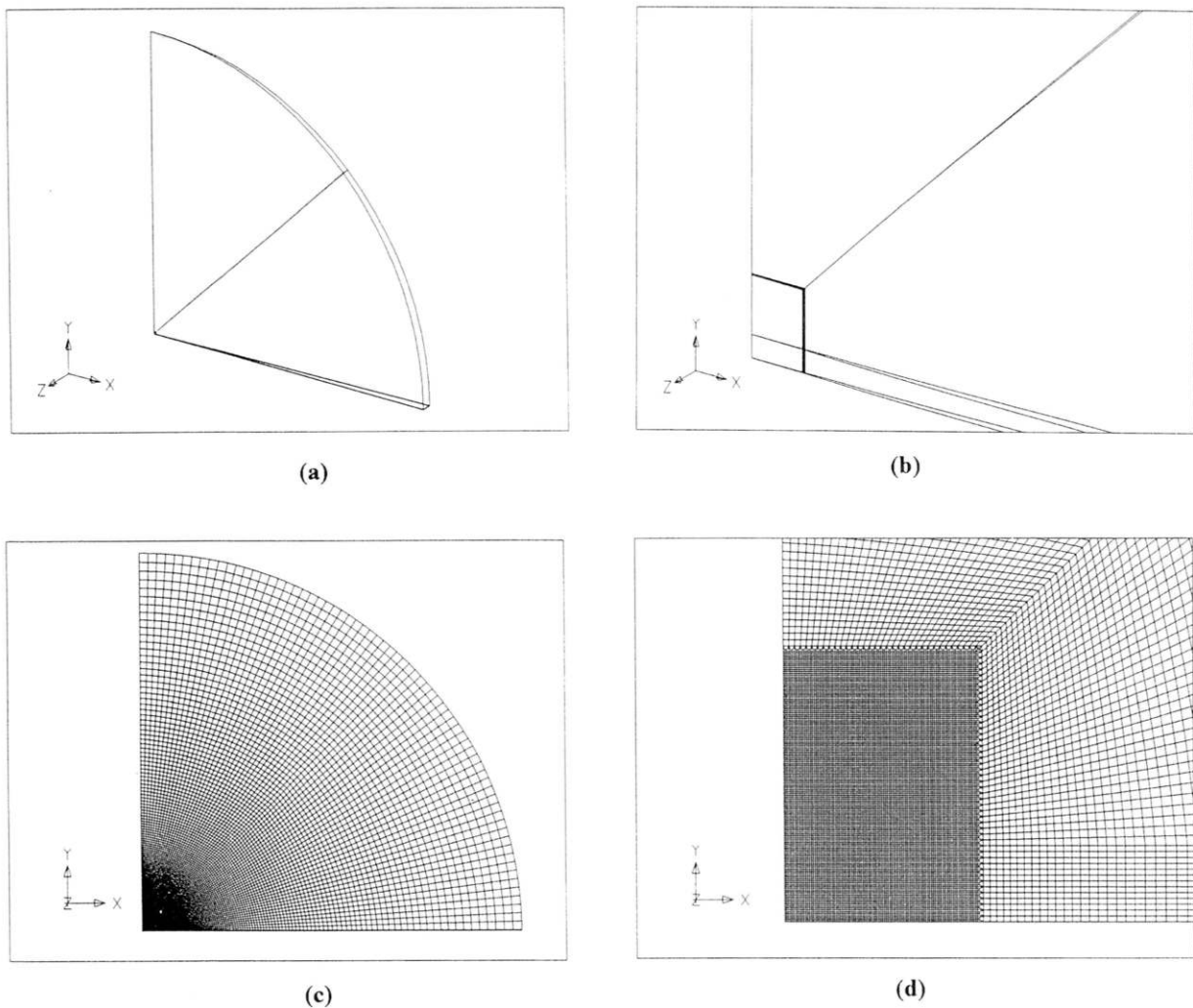
FIGURE 4 Finite element model for the bubble near the boundary problem (typical).
