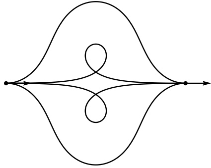
Figure 13: Optimal elasticae for (x_1, y_1, \theta_1) = (x_*, 0, 0)
