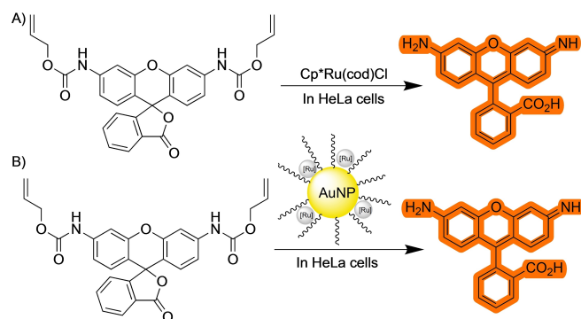
Scheme 14. Ruthenium-catalyzed deallyloxylation.
