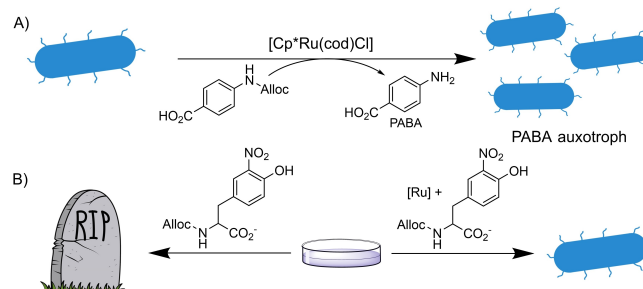
Scheme 16. Deallylation as a mean for bacterial cell survival.
