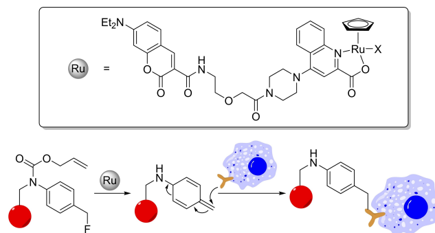
Scheme 15. Cell tagging through Ru-catalyzed deallylation.
